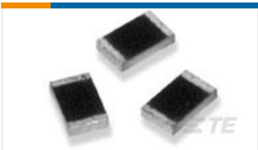
TE Part #6-1879743-8 RP 1J 23R7 0.1% 15PPM CUT LENGTH
