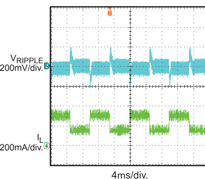
Load Transient
