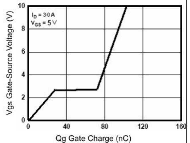
Figure 6: Gate-Charge Characteristics
