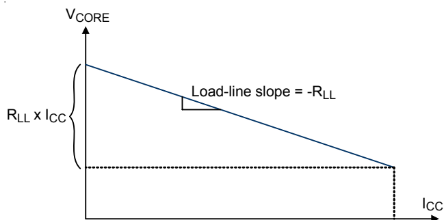
Figure 6. Load-Line (Droop)
