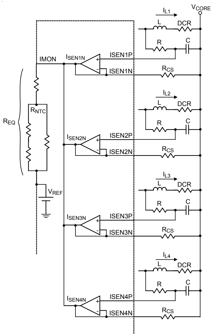
Figure 5. Total Current Sense Method
