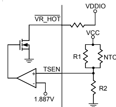
Figure 20. VR_HOT Circuit
