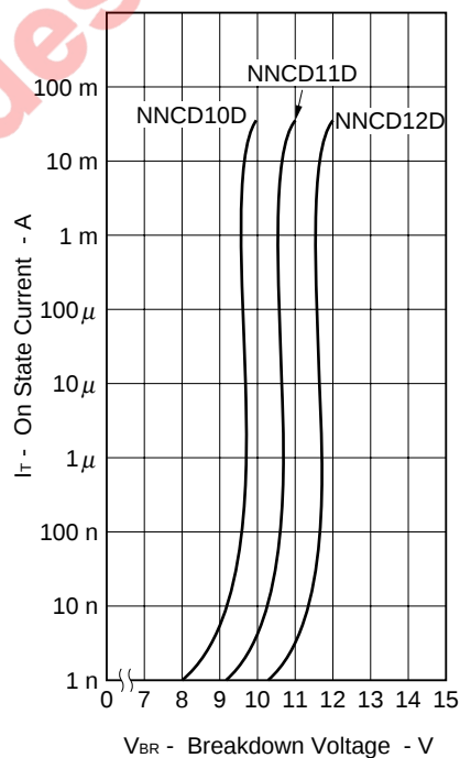
Fig. 3 I_T - V_{BR} CHARACTERISTICS
