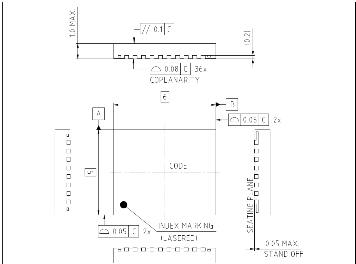
Figure 30 Package view
