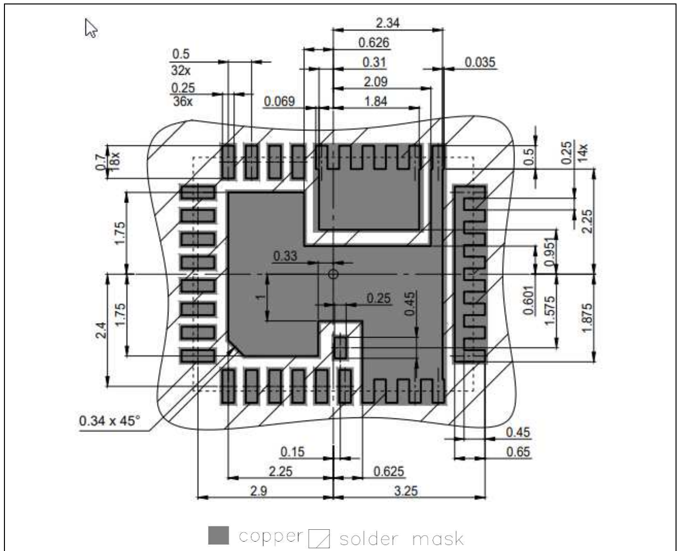
Figure 27 Solder resist
