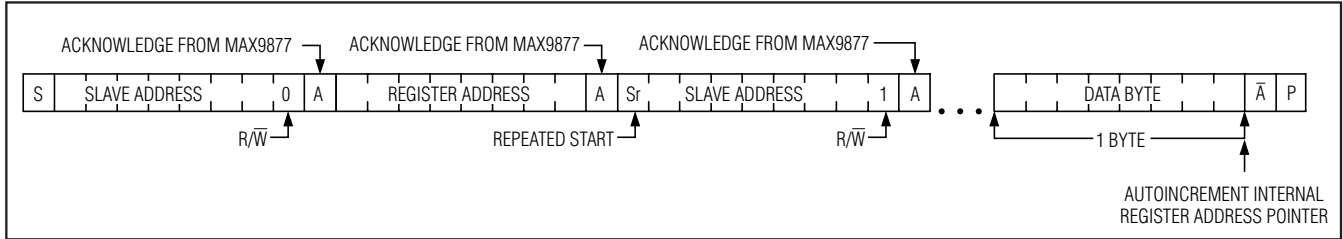
Figure 12. Reading n-Bytes of Indexed Data from the MAX9877
