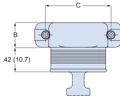
STYLE S - SIDE ENTRY
