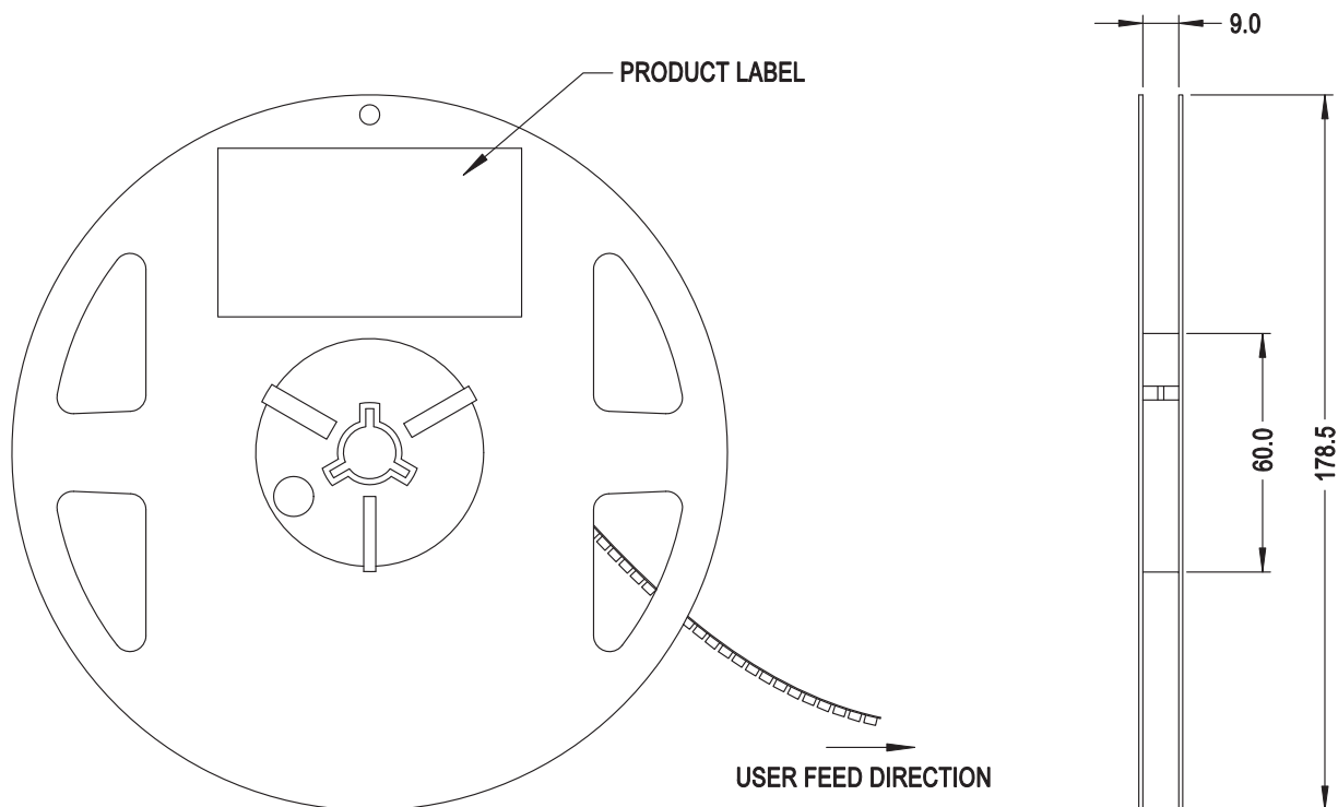
Figure 12: Reel Dimensions
