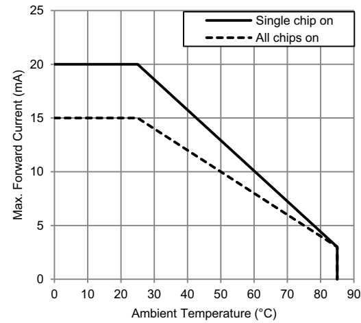
Figure 9: Derating Curve
