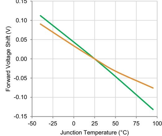
Figure 6: Forward Voltage Shift vs. Junction Temperature
