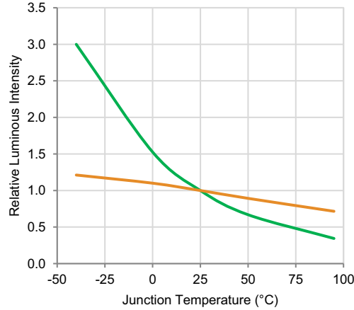
Figure 5: Relative Luminous Intensity vs. Junction Temperature
