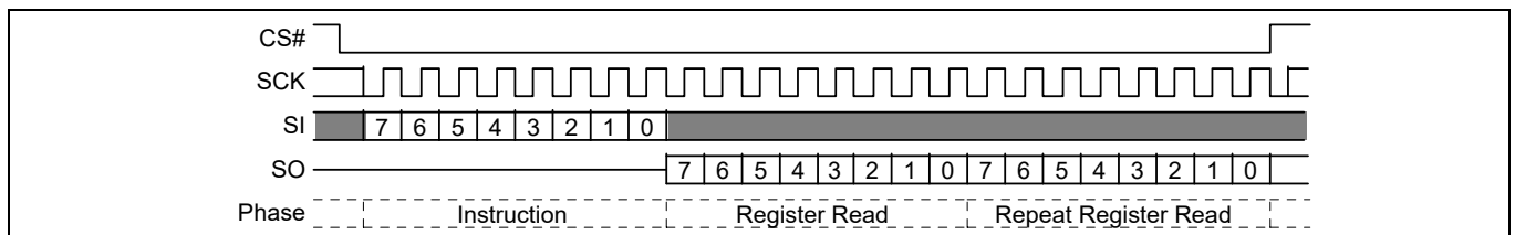
Figure 58 DLP Read (DLPRD) command sequence
