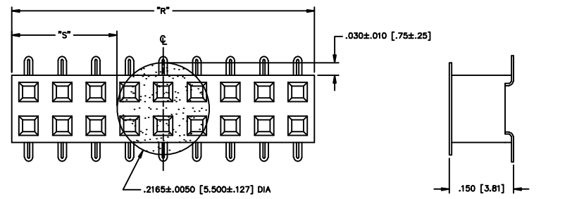
FIG. 3 -P: PICK AND PLACE PAD (PLACE PPP-03 ABOUT C.L. AS SHOWN) (SEE NOTE 10)
