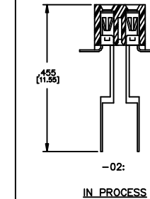
FIG. 2 -02: SURFACE MOUNT
