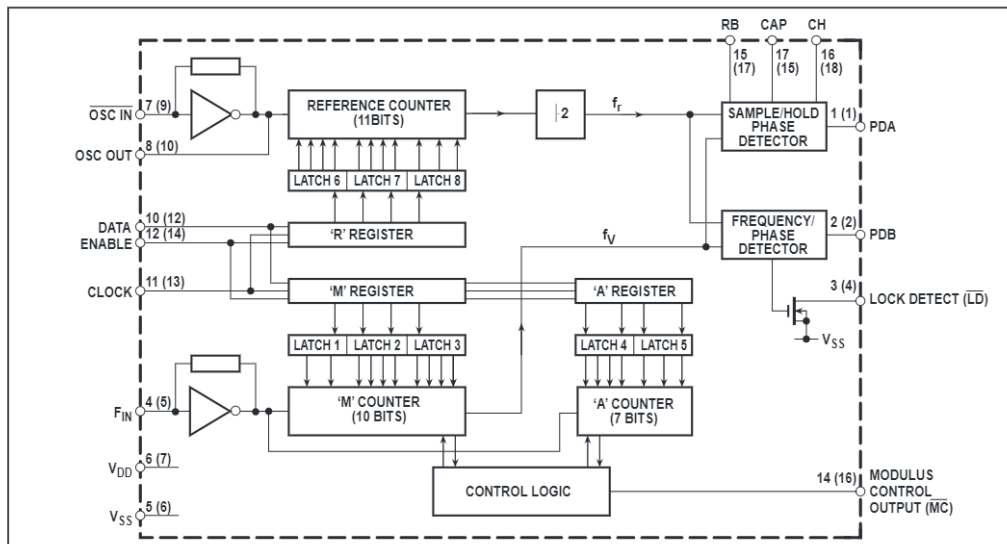
Fig.2 Block diagram (MP pinout shown in parentheses)
