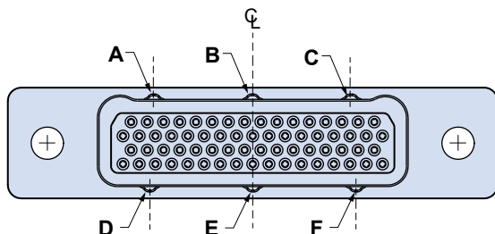
MOD-555 KEY LOCATIONS PLUG CONNECTOR MATING FACE
