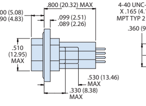
SHELL H & L
