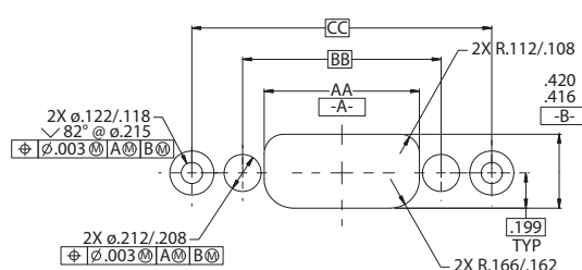
SHELL SIZES A, B, C, D, E, F, J, & K FOR DIMENSIONS, USE TABLE IV
