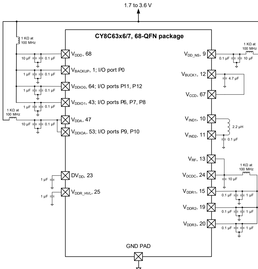
Figure 14. 68-QFN Power Connection Diagram
