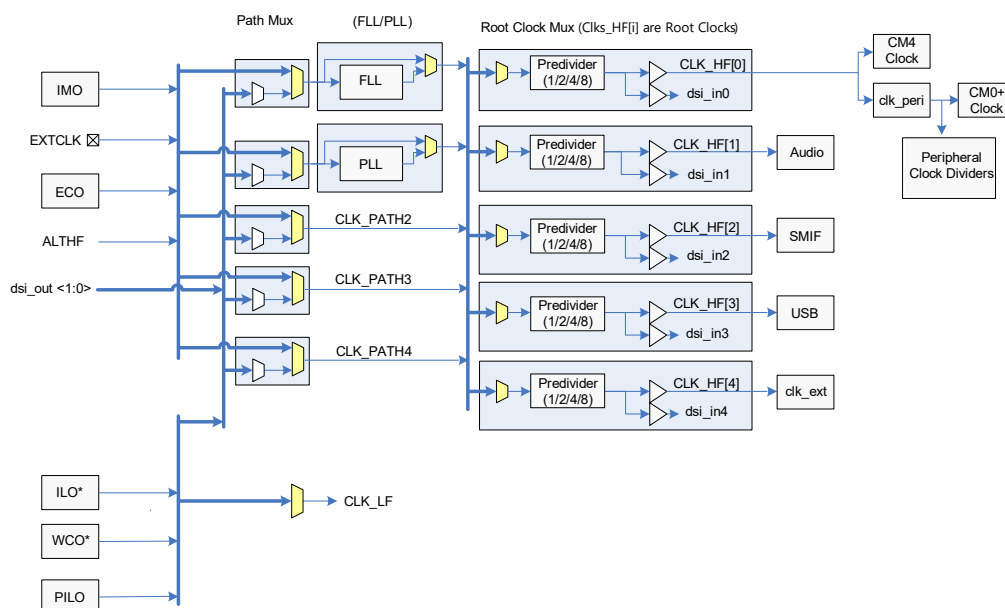
Figure 4. Clocking Diagram
