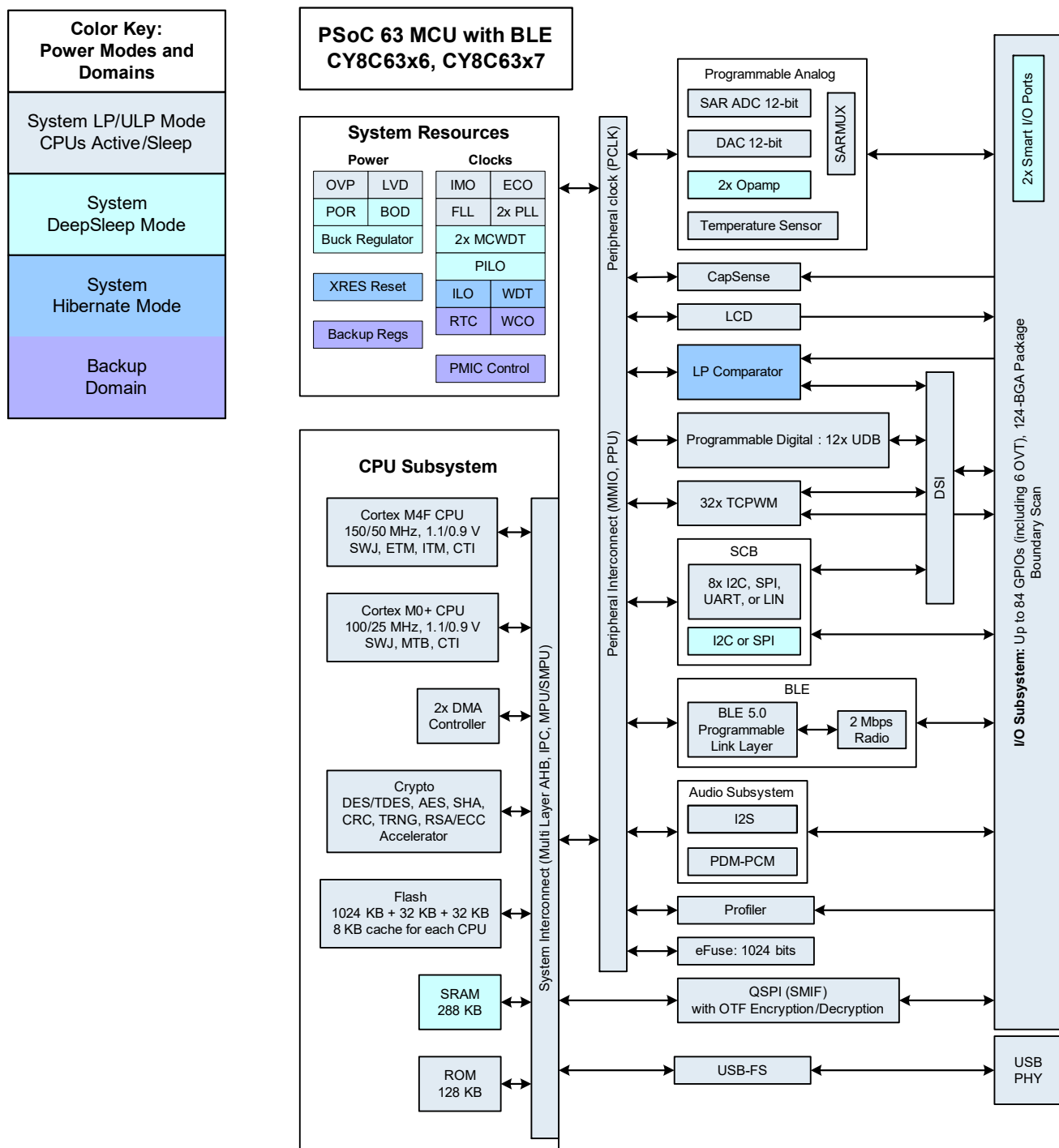
Figure 3. Block Diagram
