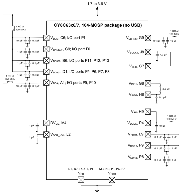
Figure 12. 104-MCSP Power Connection Diagram
