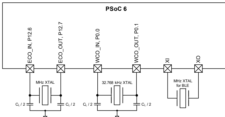
Figure 5. Oscillator Circuits
