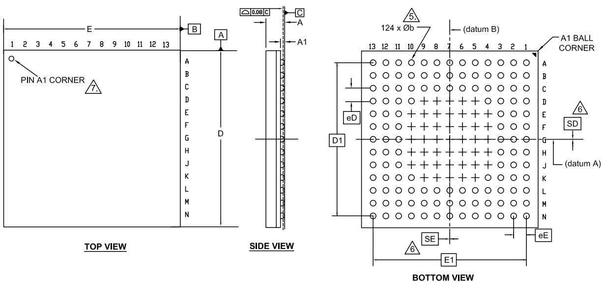
Figure 18. 124-BGA 9.0 × 9.0 × 1.0 mm
