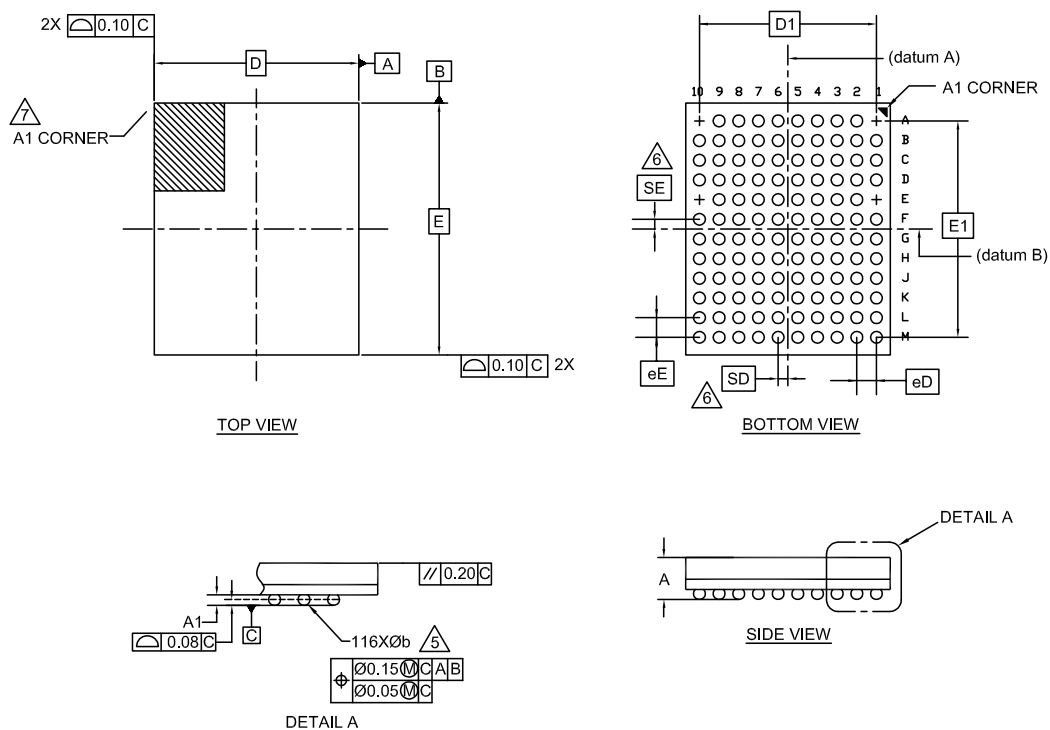
Figure 17. 116-BGA 5.2 × 6.4 × 0.70 mm
