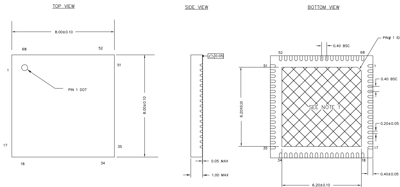
Figure 19. 68 QFN 8 × 8 × 1 mm
