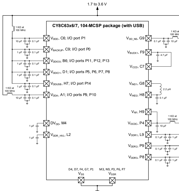
Figure 13. 104-MCSP-USB Power Connection Diagram
