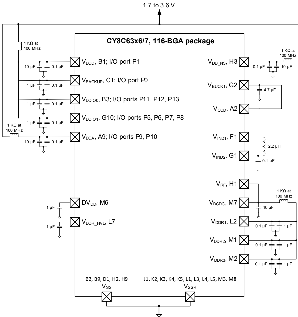
Figure 11. 116-BGA Power Connection Diagram
