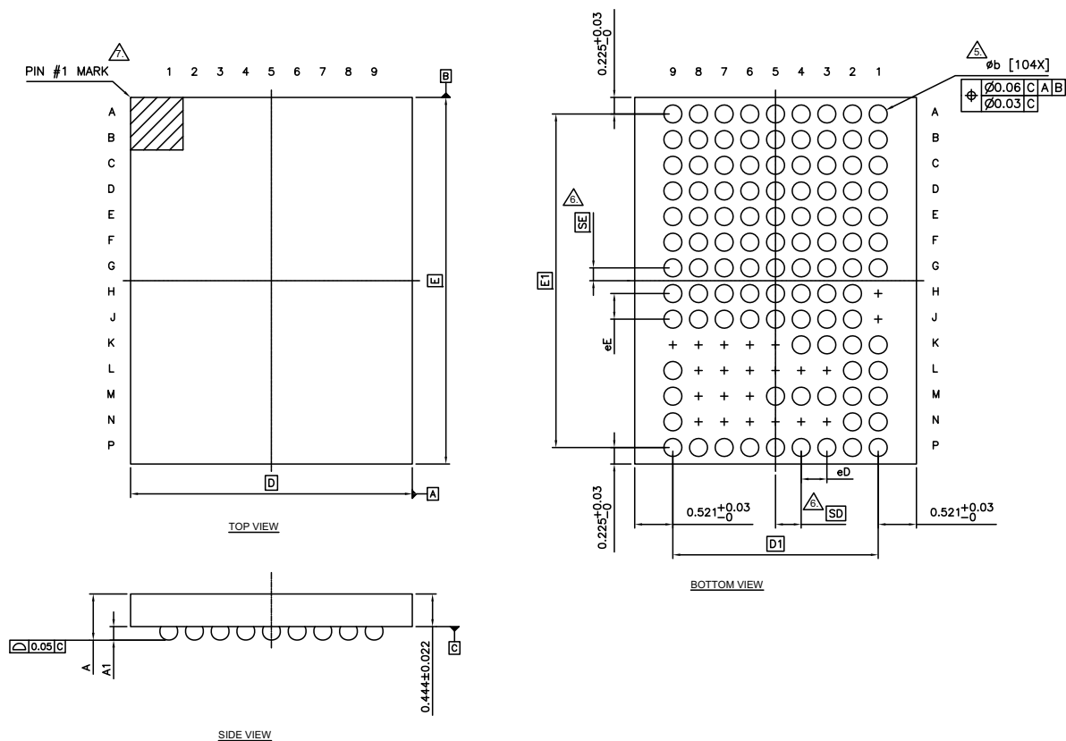
Figure 16. 104-WLCSP 3.8 × 5.0 × 0.65 mm
