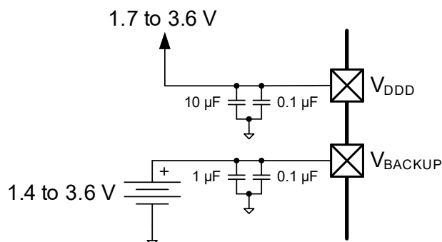
Figure 15. Separate Battery Connection to V_{\text{BACKUP}}
