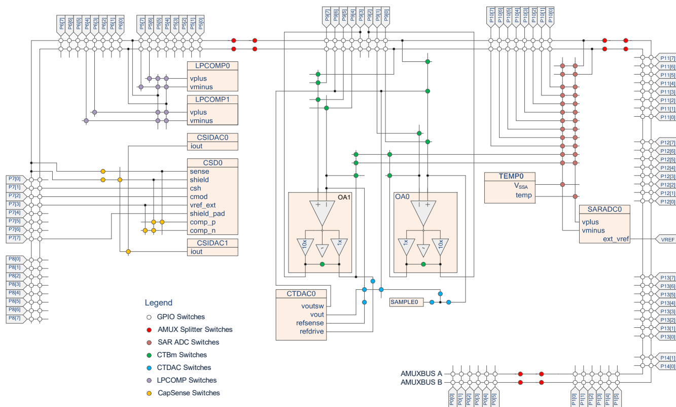
Figure 6. Analog Subsystem
