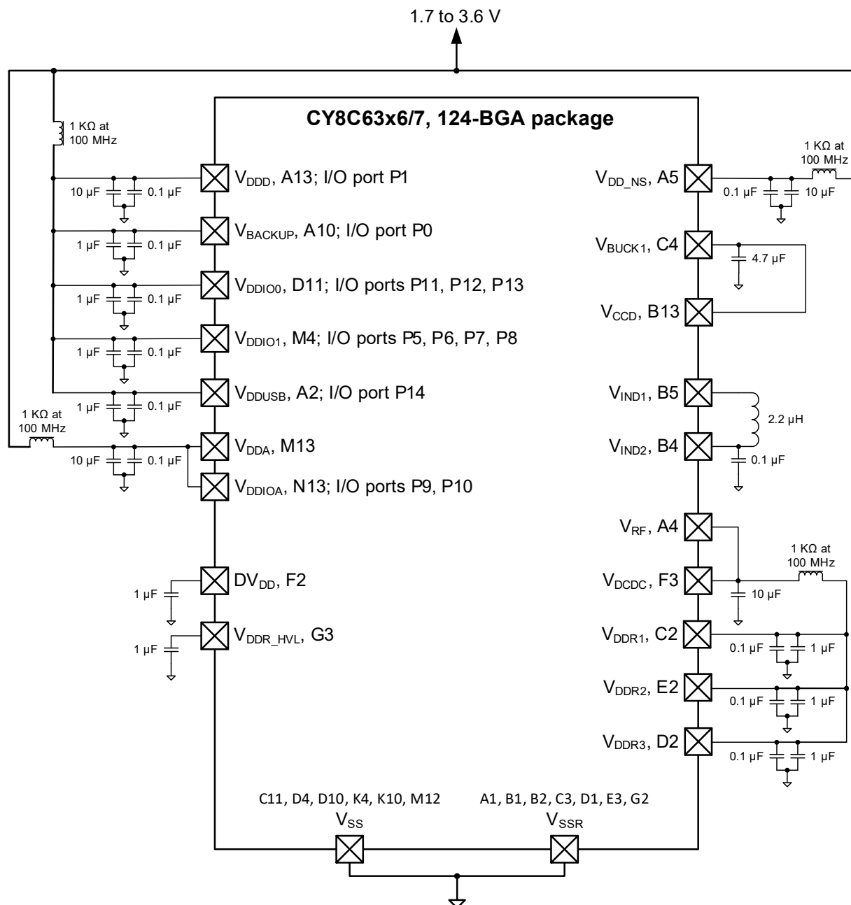
Figure 10. 124-BGA Power Connection Diagram
