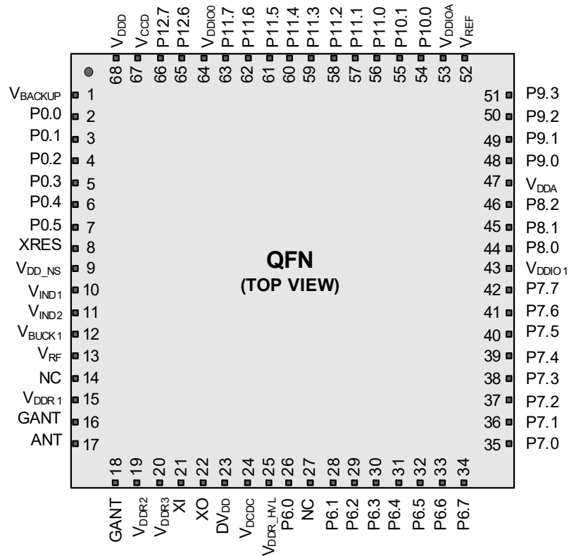
Figure 9. Device Pinout for 68-QFN Package [1]
