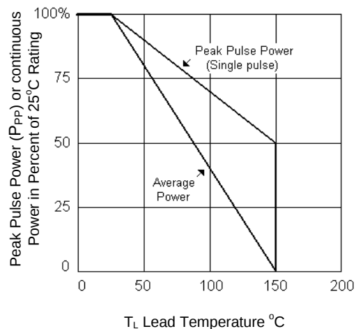
FIGURE 4 Derating
