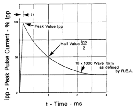
Test waveform parameters: t_r=10 \mu s , t_p=1000 \mu s
