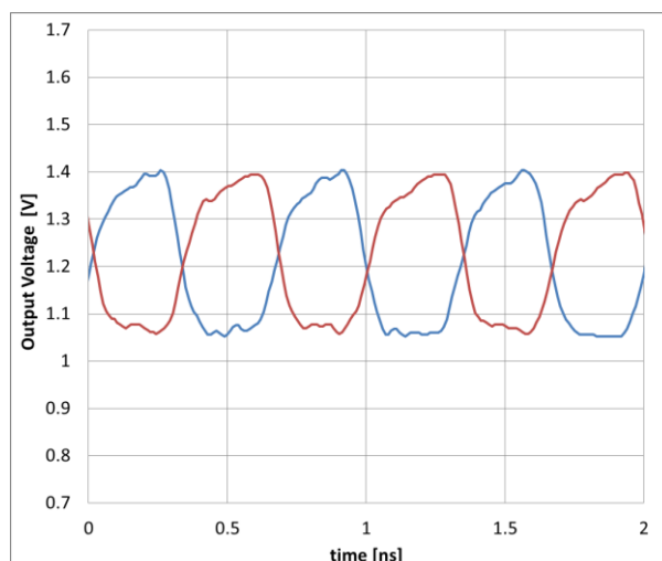
Figure 22. 1.5GHz LVDS
