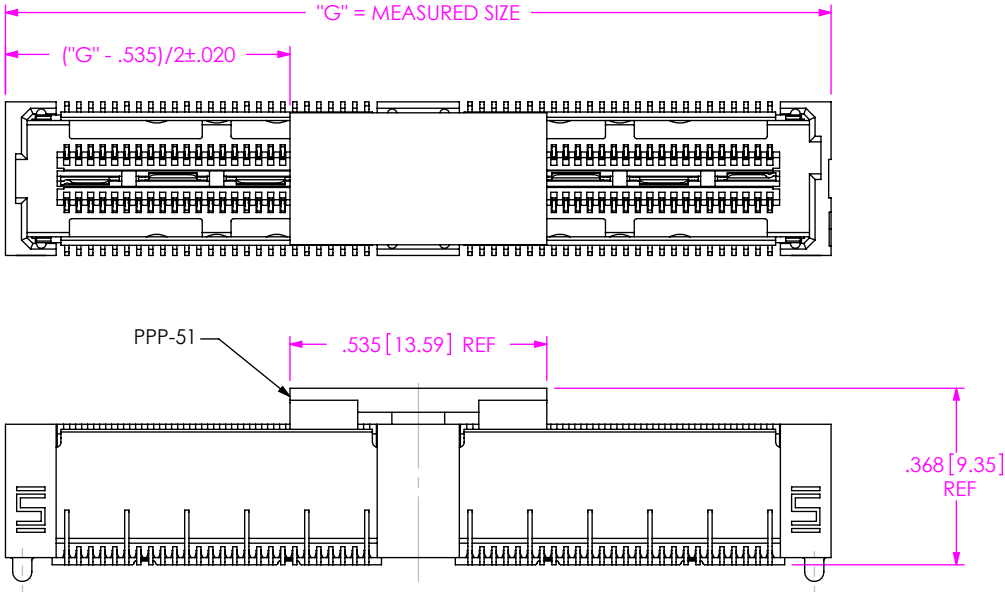
FIG 4 -P: PICK & PLACE PAD OPTION
