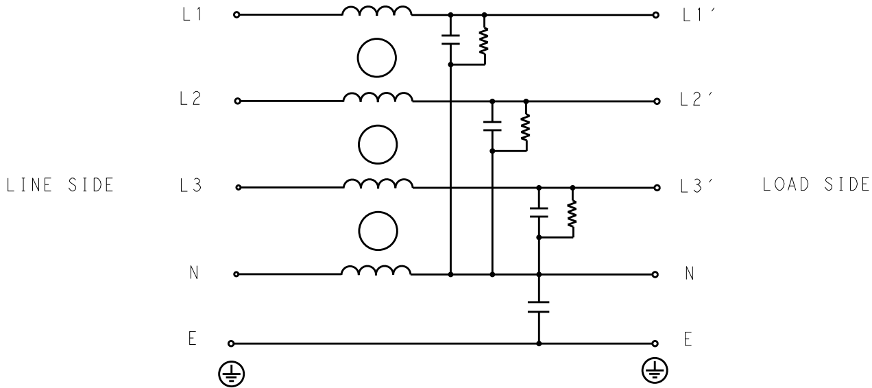
SCHEMATIC
