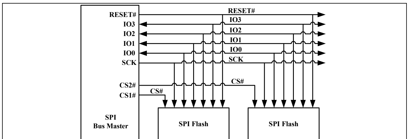
Figure 9 Bus master and memory devices on the SPI bus - quad bit data path - Separate RESET#
