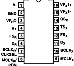
CD22354A, CD22357A (PDIP) TOP VIEW
