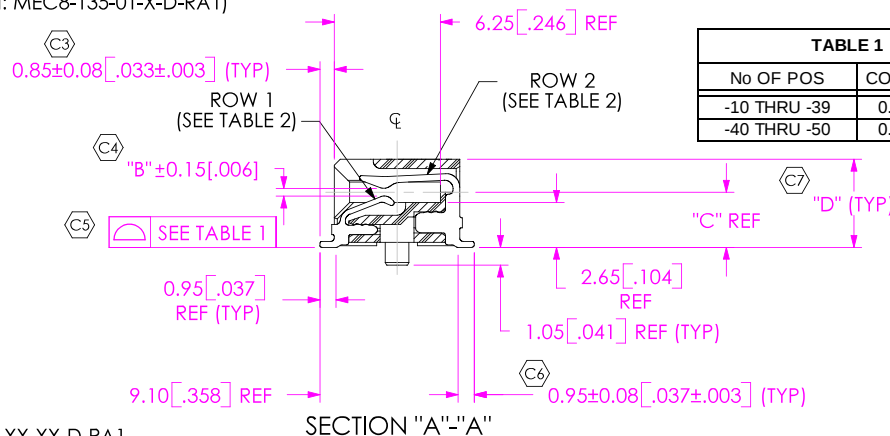
FIG. 1 FOR POSITIONS -10, -20, -30 & -35 (SHOWN: MEC8-135-01-X-D-RA1)
