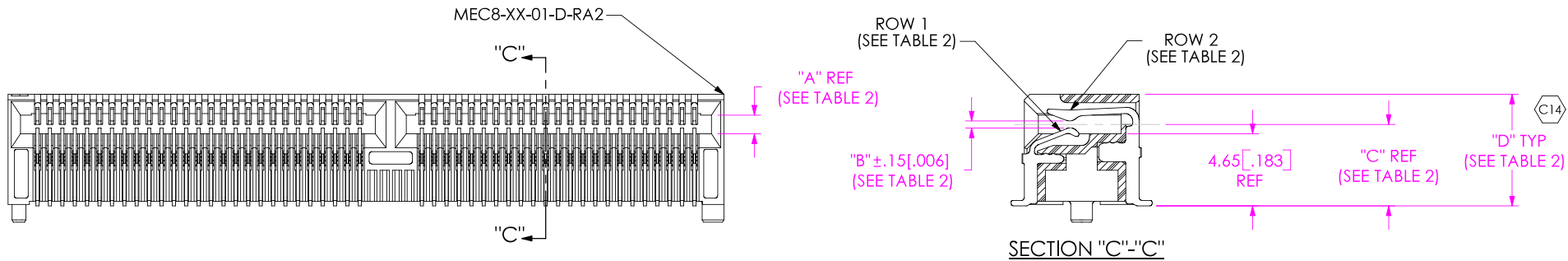
FIG. 3 -RA2: ELEVATED OPTION (SAME AS FIG. 2, UNLESS OTHERWISE STATED) (SHOWN: MEC8-150-01-X-D-RA2) * = NOT TOOLED
