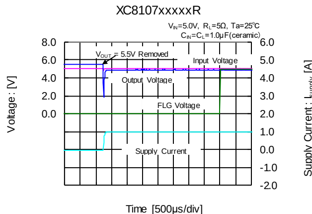
(40) Reverse Voltage Released Voltage ( C_L=1.0\mu\text{F} )
