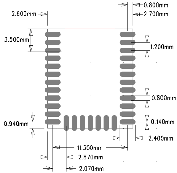
Figure 8.4. BGM111E Recommended PCB Land Pattern
