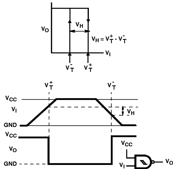
FIGURE 3. HYSTERESIS DEFINITION, CHARACTERISTIC, AND TEST SET-UP
