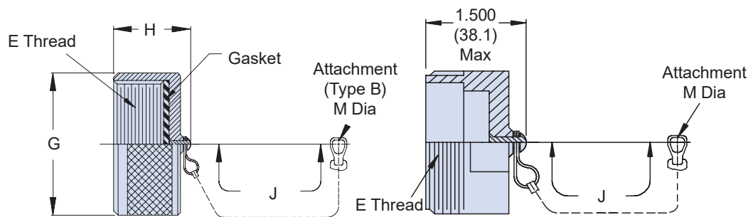
MS17349 Receptacle Cover
