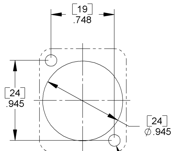
PANEL CUT-OUT FRONT OR REAR MOUNT
