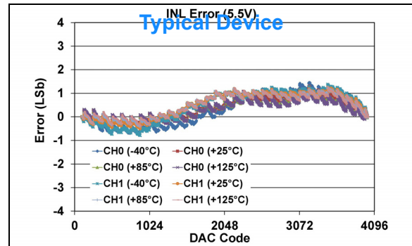
FIGURE 1-149: INL Error vs. DAC Code, and Temperature (Code 100 - 4000) (Dual Channel - MCP47FXB22 ) ( 12-bit: V_{DD} = 5.5\text{V} , V_{REF} = V_{DD} , VRxB:VRxA = '11' ( V_{REF} Buffered), Gx = '0' (1x)).
