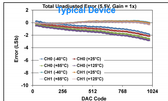
FIGURE 1-378: Total Unadjusted Error ( V_{OUT} ) vs. DAC Code, and Temperature (Dual Channel - MCP47FXB12 ) ( 10-bit: V_{DD} = 5.5\text{V} , V_{REF} = 2.048\text{V} , VRxB:VRxA = '11' ( V_{REF} Buffered), Gx = '0' (1x)).
