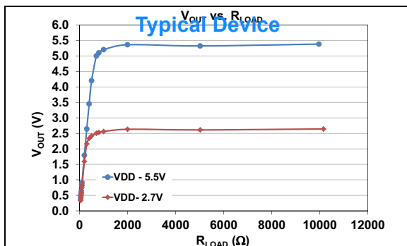
FIGURE 1-30: V_{OUT} vs. R_{LOAD} and Voltage (at +25^\circ\text{C} )
