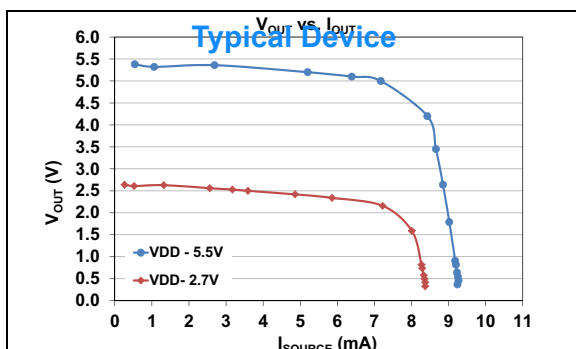
FIGURE 1-29: V_{OUT} vs. I_{OUT} and Voltage (at +25^\circ\text{C} )
