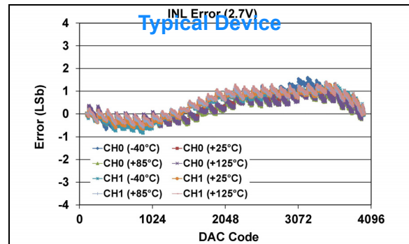
FIGURE 1-150: INL Error vs. DAC Code, and Temperature (Code 100 - 4000) (Dual Channel - MCP47FXB22 ) ( 12-bit: V_{DD} = 2.7\text{V} , V_{REF} = V_{DD} , VRxB:VRxA = '11' ( V_{REF} Buffered), Gx = '0' (1x)).
