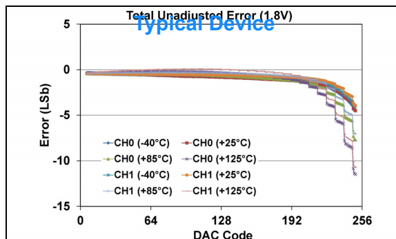
FIGURE 1-397: Total Unadjusted Error ( V_{OUT} ) vs. DAC Code, and Temperature (Dual Channel - MCP47FXB02 ) ( 8-bit: V_{DD} = 1.8\text{V} , VRxB:VRxA = '00' ( V_{DD} ), Gx = '0' (1x)) (see Appendix B.1 for additional information).
