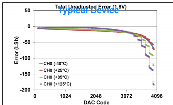
FIGURE 1-34: Total Unadjusted Error ( V_{OUT} ) vs. DAC Code, and Temperature (Single Channel - MCP47FXB21 ) (12-bit: V_{DD} = 1.8\text{V} , VRxB:VRxA = '00' ( V_{DD} ), Gx = '0' (1x)) (see Appendix B.1 for additional information).
