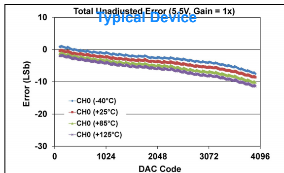
FIGURE 1-195: Total Unadjusted Error ( V_{OUT} ) vs. DAC Code, and Temperature (Single Channel - MCP47FXB21) (12-bit: V_{DD} = 5.5\text{V} , V_{REF} = 2.048\text{V} , VRxB:VRxA = '11' ( V_{REF} Buffered), Gx = '0' (1x)).
