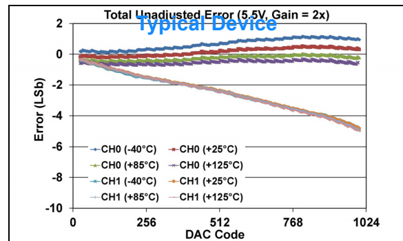
FIGURE 1-377: Total Unadjusted Error ( V_{OUT} ) vs. DAC Code, and Temperature (Dual Channel - MCP47FXB12 ) ( 10-bit: V_{DD} = 5.5\text{V} , V_{REF} = 2.048\text{V} , VRxB:VRxA = '11' ( V_{REF} Buffered), Gx = '1' (2x)).
