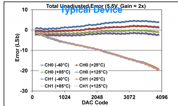
FIGURE 1-197: Total Unadjusted Error ( V_{OUT} ) vs. DAC Code, and Temperature (Dual Channel - MCP47FXB22) (12-bit: V_{DD} = 5.5\text{V} , V_{REF} = 2.048\text{V} , VRxB:VRxA = '11' ( V_{REF} Buffered), Gx = '1' (2x)).
