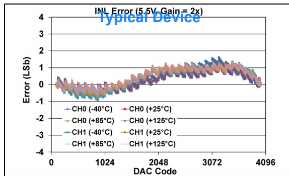
FIGURE 1-131: INL Error vs. DAC Code, and Temperature (Code 100 - 4000) (Dual Channel - MCP47FXB22) (12-bit: V_{DD} = 5.5\text{V} , V_{REF} = 2.048\text{V} , VRxB:VRxA = '10' ( V_{REF} Unbuffered), Gx = '1' (2x)).
