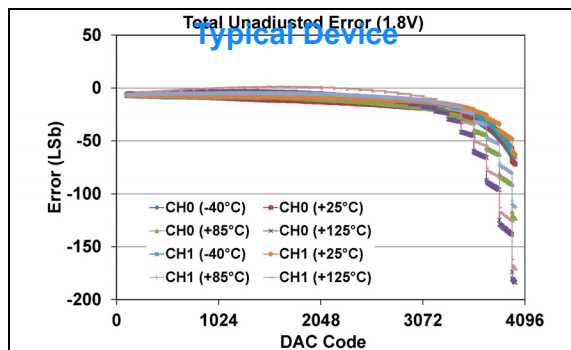
FIGURE 1-37: Total Unadjusted Error ( V_{OUT} ) vs. DAC Code, and Temperature (Dual Channel - MCP47FXB22 ) (12-bit: V_{DD} = 1.8\text{V} , VRxB:VRxA = '00' ( V_{DD} ), Gx = '0' (1x)) (see Appendix B.1 for additional information).
