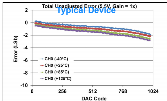
FIGURE 1-375: Total Unadjusted Error ( V_{OUT} ) vs. DAC Code, and Temperature (Single Channel - MCP47FXB11 ) ( 10-bit: V_{DD} = 5.5\text{V} , V_{REF} = 2.048\text{V} , VRxB:VRxA = '11' ( V_{REF} Buffered), Gx = '0' (1x)).
