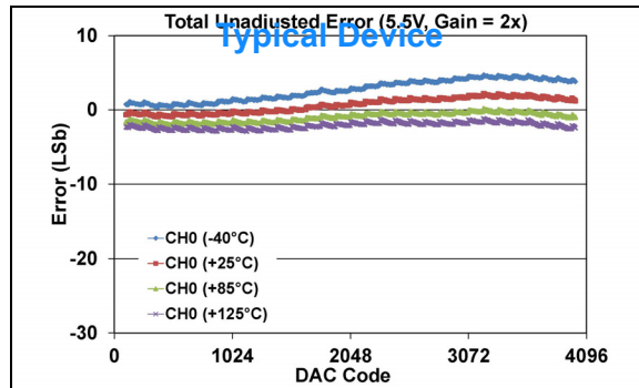
FIGURE 1-194: Total Unadjusted Error ( V_{OUT} ) vs. DAC Code, and Temperature (Single Channel - MCP47FXB21) (12-bit: V_{DD} = 5.5\text{V} , V_{REF} = 2.048\text{V} , VRxB:VRxA = '11' ( V_{REF} Buffered), Gx = '1' (2x)).
