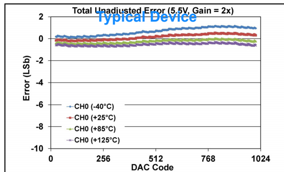
FIGURE 1-374: Total Unadjusted Error ( V_{OUT} ) vs. DAC Code, and Temperature (Single Channel - MCP47FXB11 ) ( 10-bit: V_{DD} = 5.5\text{V} , V_{REF} = 2.048\text{V} , VRxB:VRxA = '11' ( V_{REF} Buffered), Gx = '1' (2x)).
