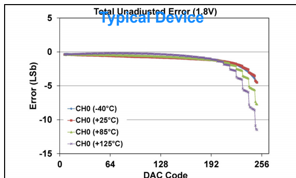
FIGURE 1-394: Total Unadjusted Error ( V_{OUT} ) vs. DAC Code, and Temperature (Single Channel - MCP47FXB01 ) ( 8-bit: V_{DD} = 1.8\text{V} , VRxB:VRxA = '00' ( V_{DD} ), Gx = '0' (1x)) (see Appendix B.1 for additional information).
