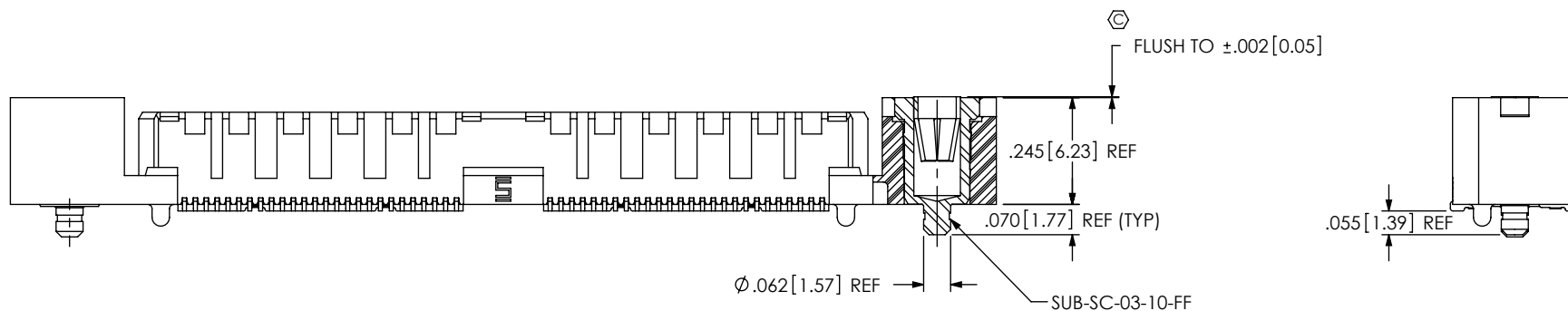
SECTION "F"-"F"
