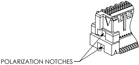
POLARIZATION NOTCHES
