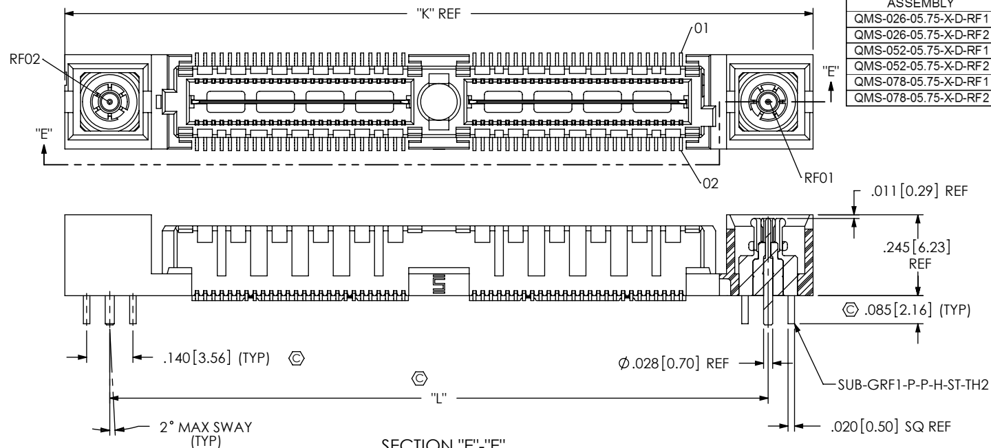
SECTION "E"-"E"
