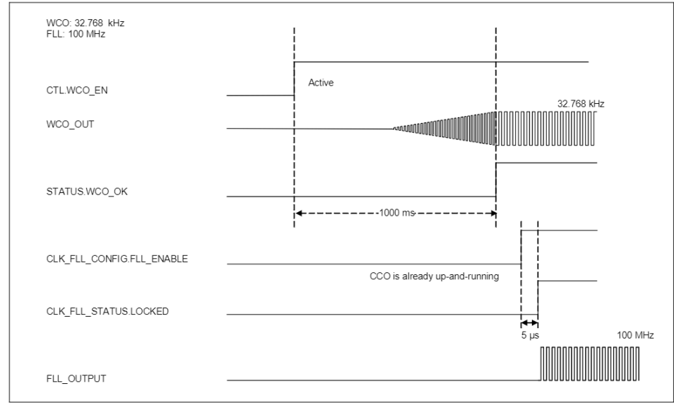
Figure 26-25 WCO to FLL diagram
