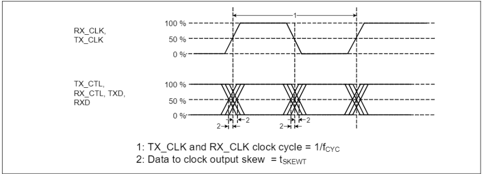
Figure 26-30 RGMII Tx timing diagram
