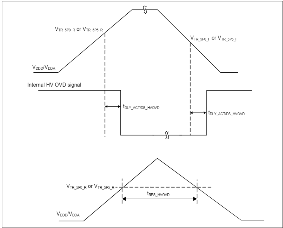
Figure 26-18 High-voltage OVD specifications
