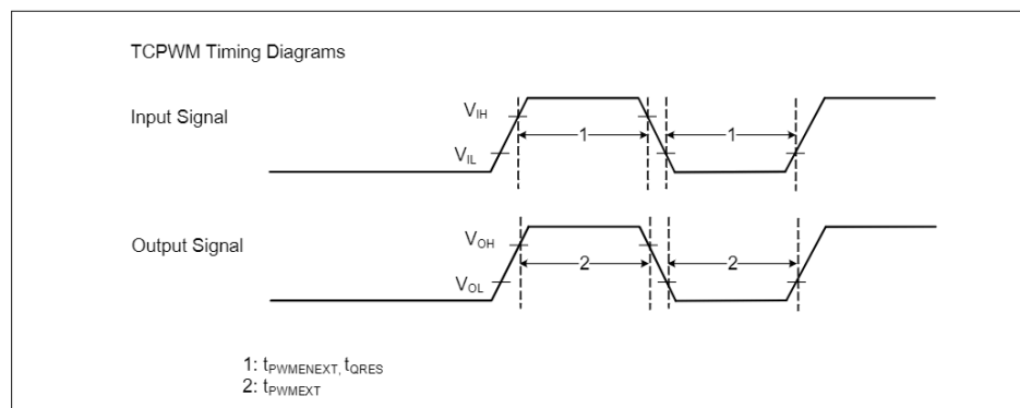
Figure 26-8 TCPWM timing diagrams
