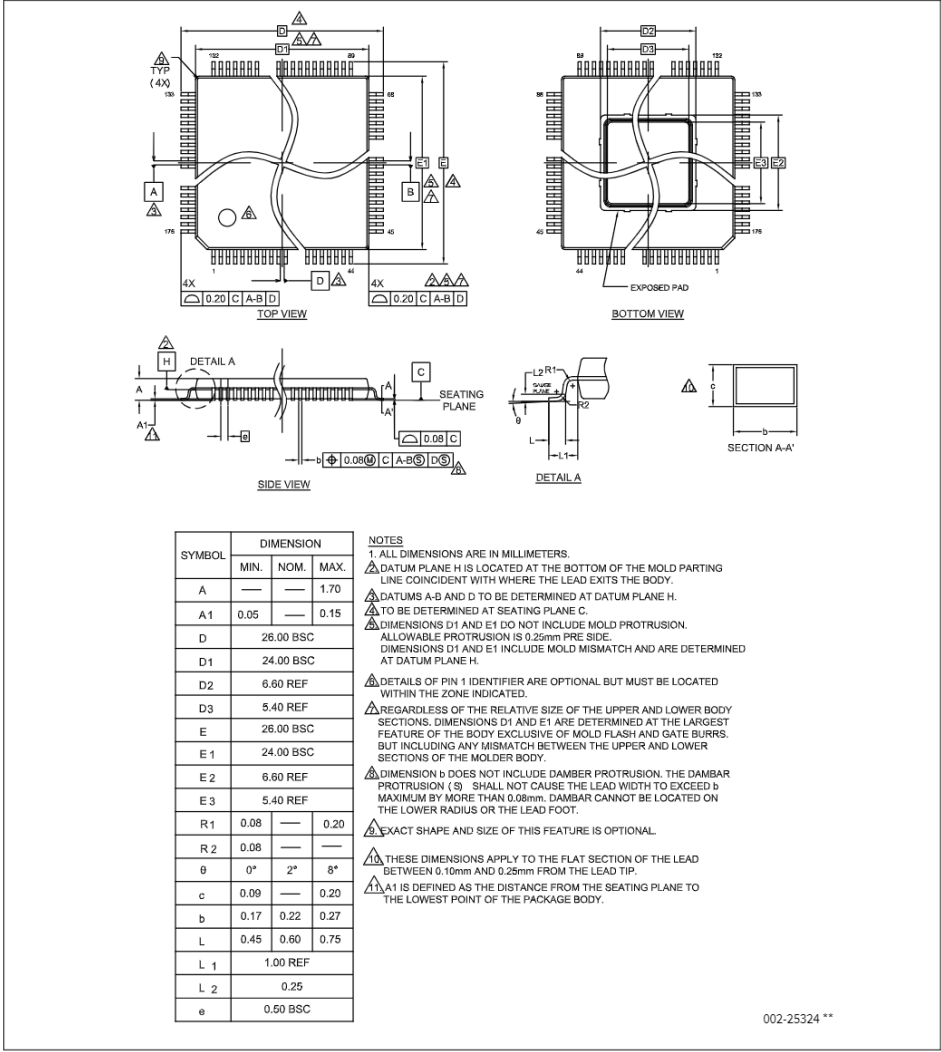
Figure 28-1 Package outline - 176-TQFP
