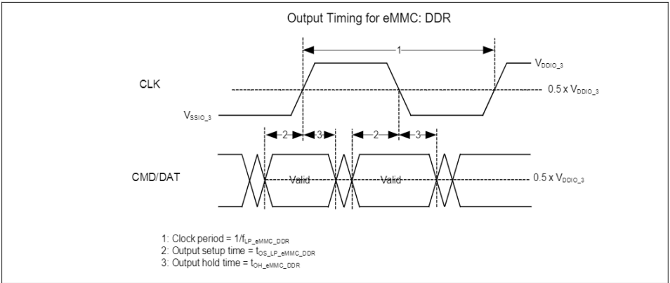
Figure 26-37 eMMC DDR output timing
