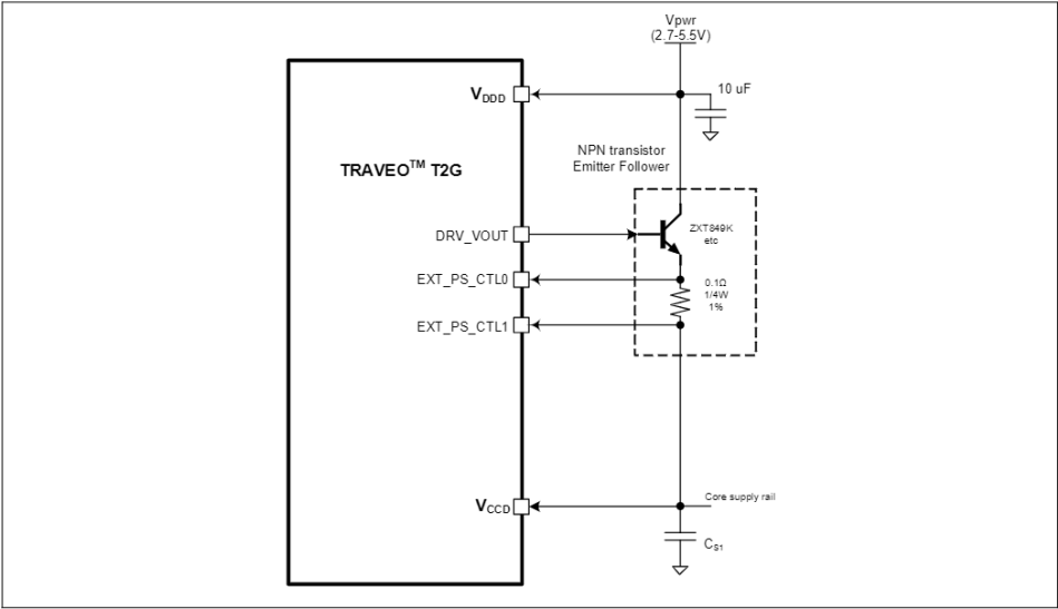
Figure 3-1 Sample core external regulator with NPN transistor
