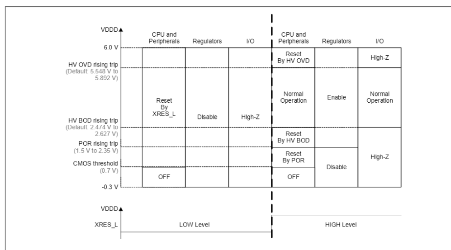
Figure 26-14 Device operations supply range
