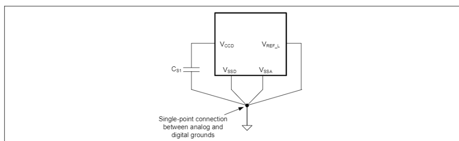
Figure 26-2 Smoothing capacitor
