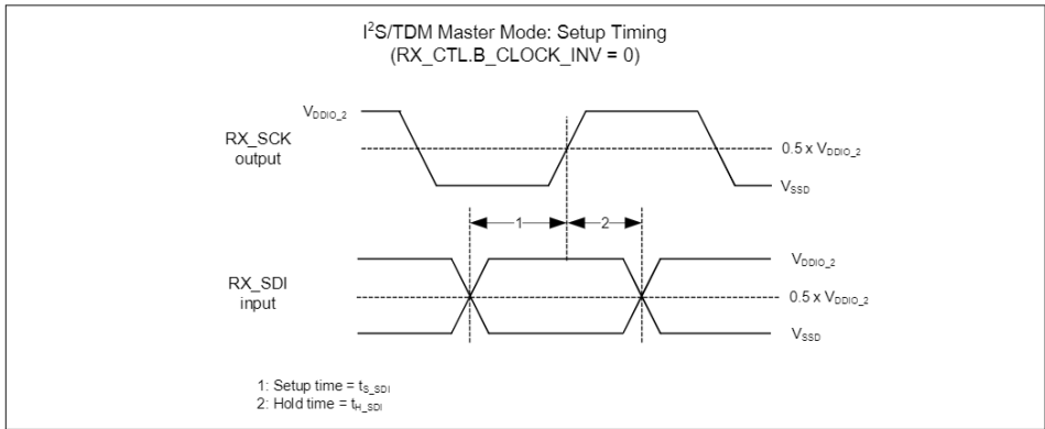
Figure 26-39 Master setup without clock inversion
