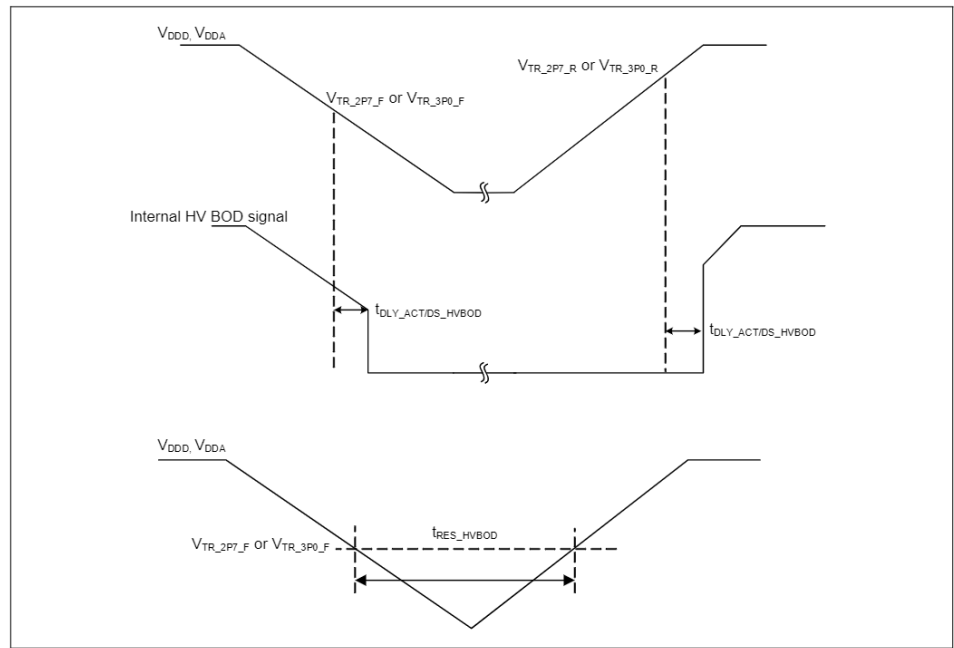
Figure 26-16 High-voltage BOD specifications
