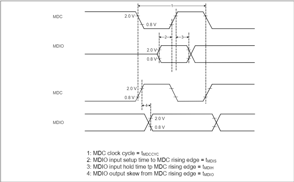
Figure 26-27 MDIO timing diagram
