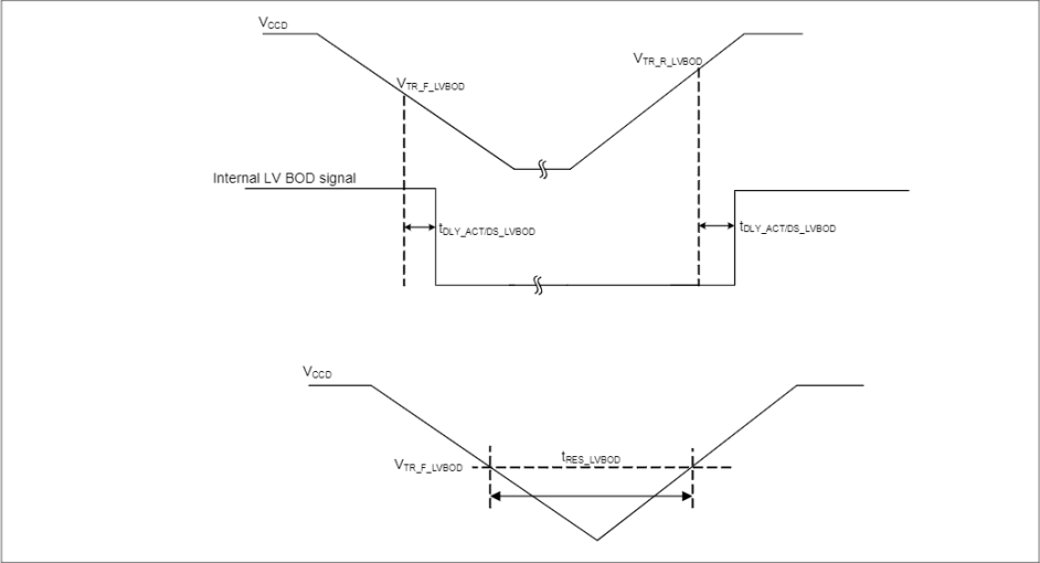
Figure 26-17 Low-voltage BOD specifications
