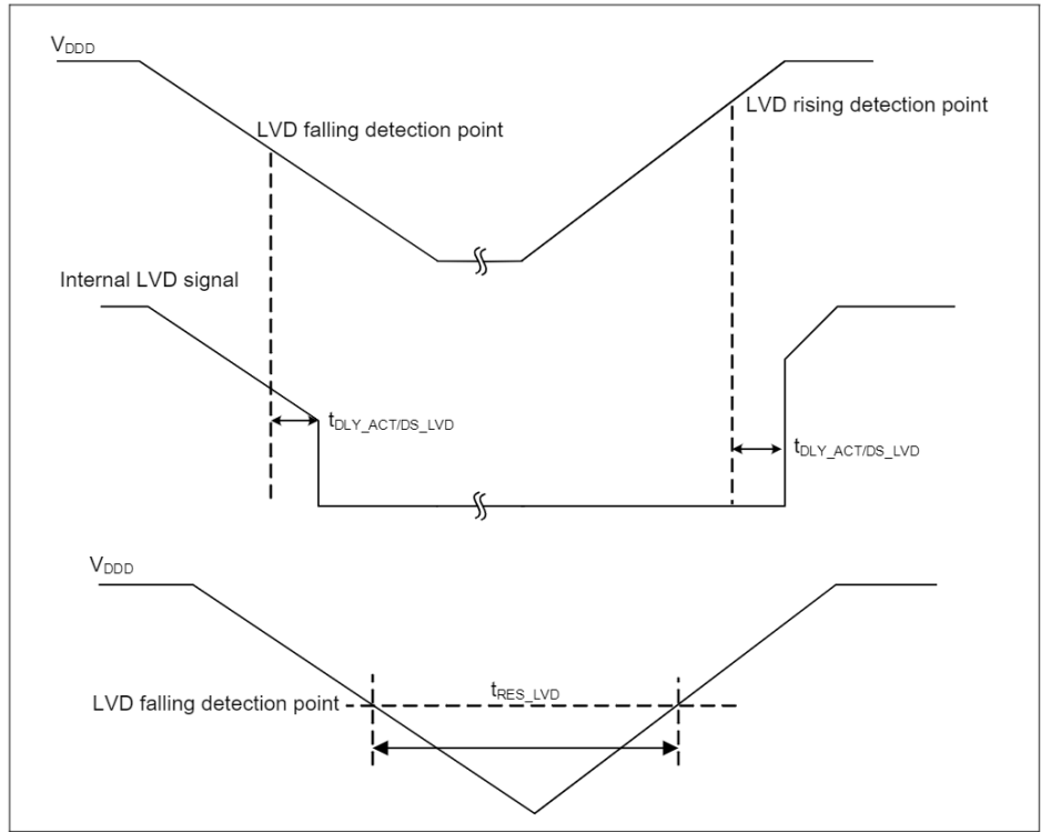
Figure 26-20 LVD specifications
