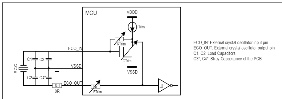
Figure 26-22 ECO connection scheme [61]
