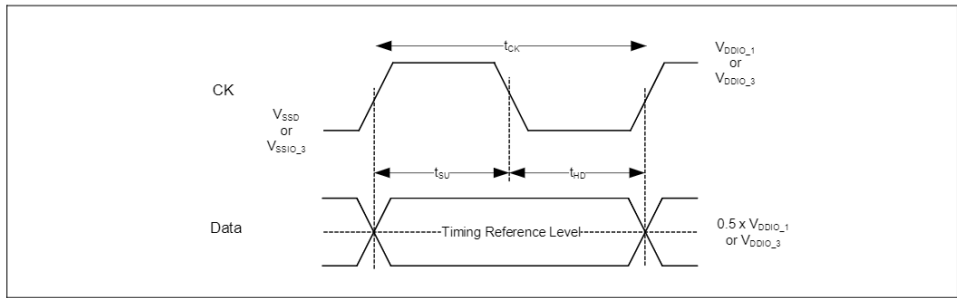
Figure 26-43 SDR write timing reference level
