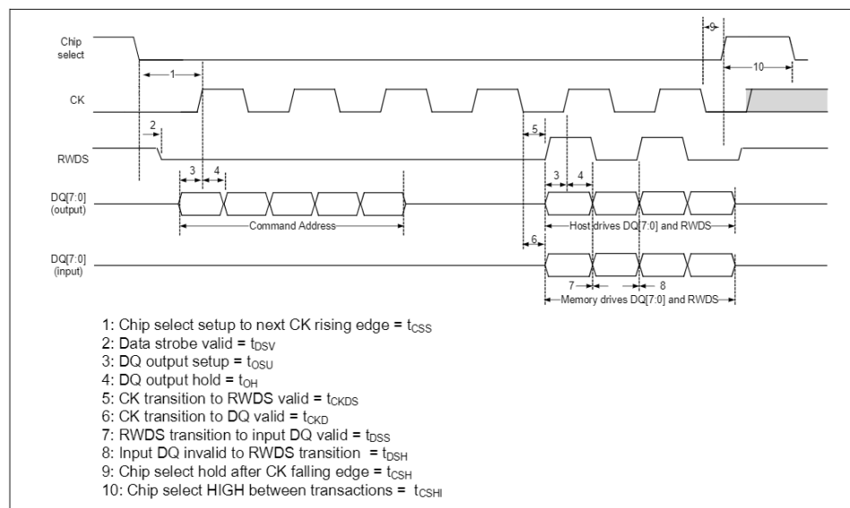
Figure 26-50 HYPERBUS™ timing diagram
