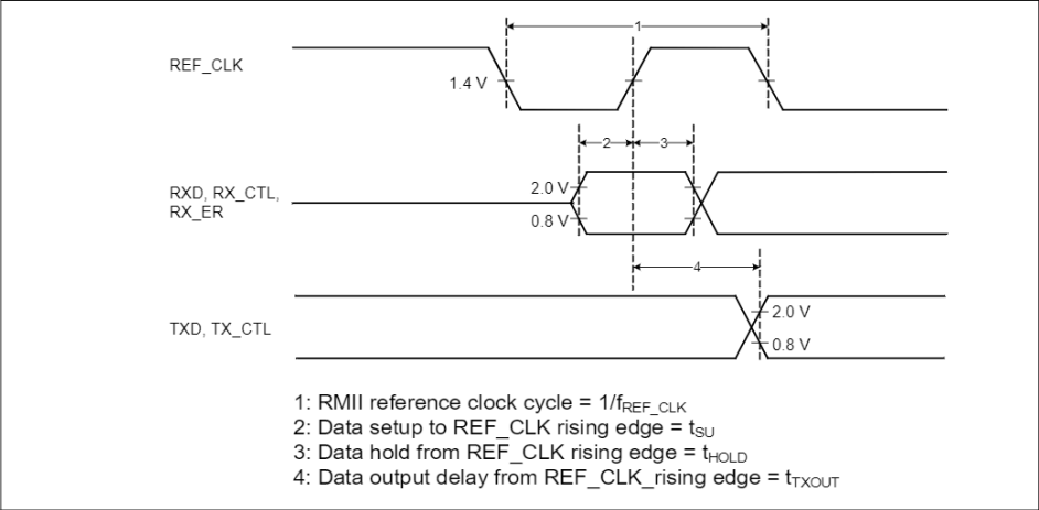
Figure 26-28 RMII timing diagram
