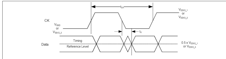
Figure 26-46 DDR read timing reference level
