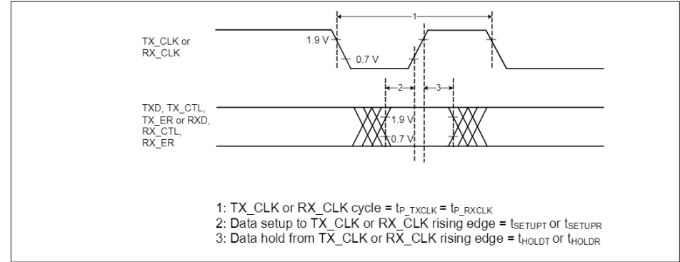
Figure 26-29 GMII timing diagram
