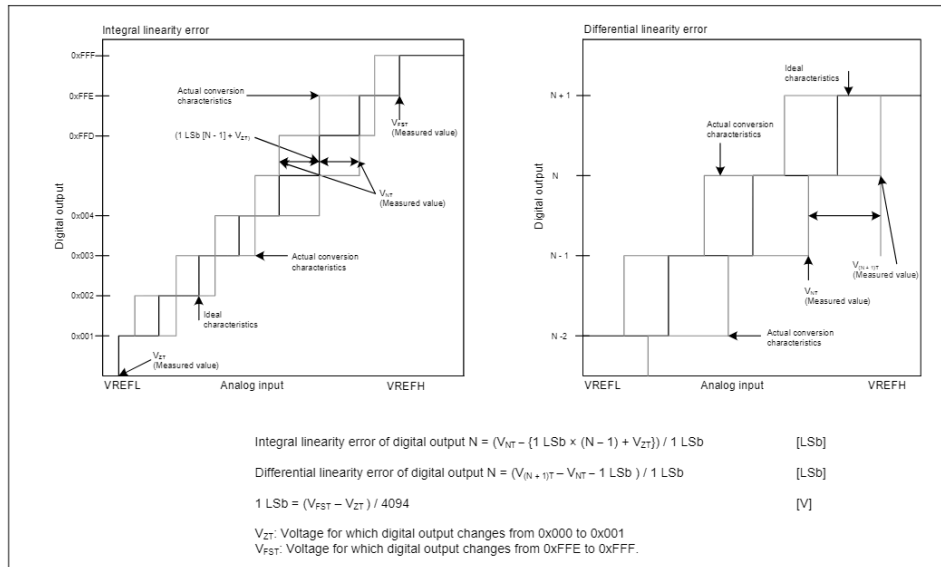
Figure 26-5 Integral and differential linearity errors
