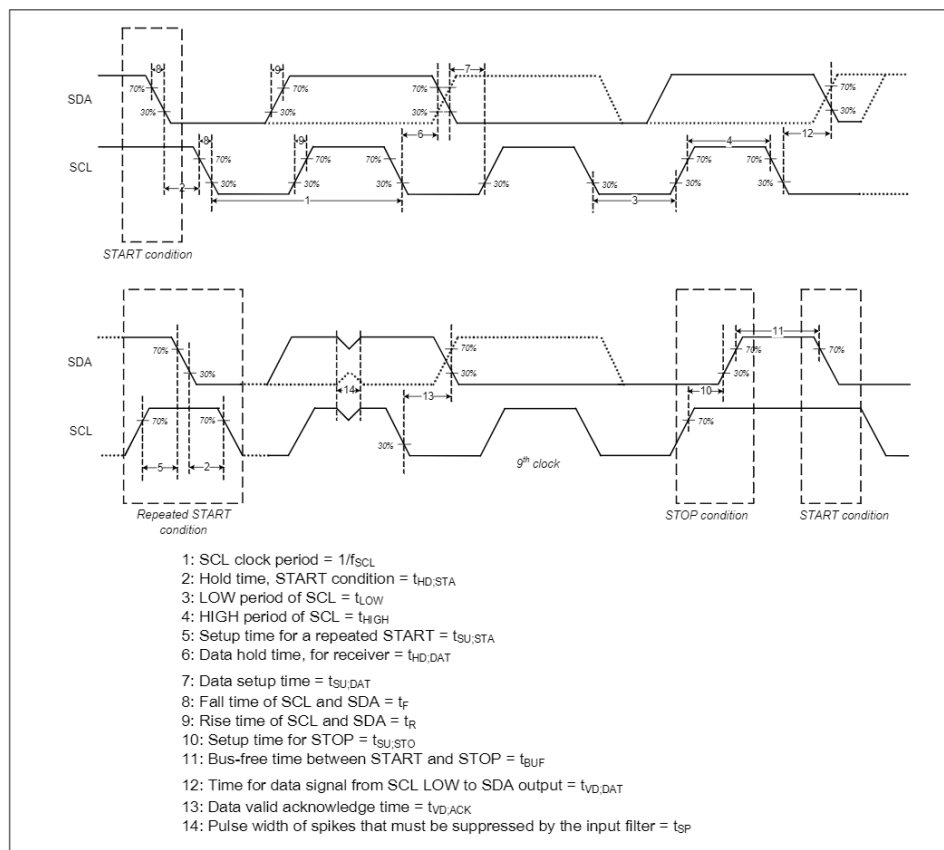
Figure 26-9 I²C timing diagrams
