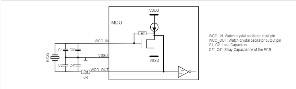
Figure 26-23 WCO connection scheme [63]
