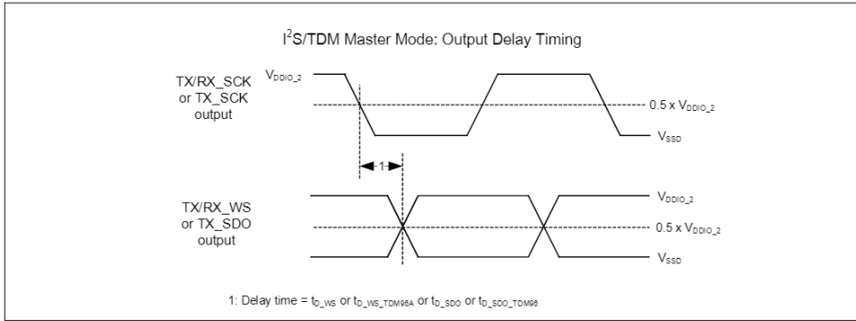
Figure 26-38 Master output delay
