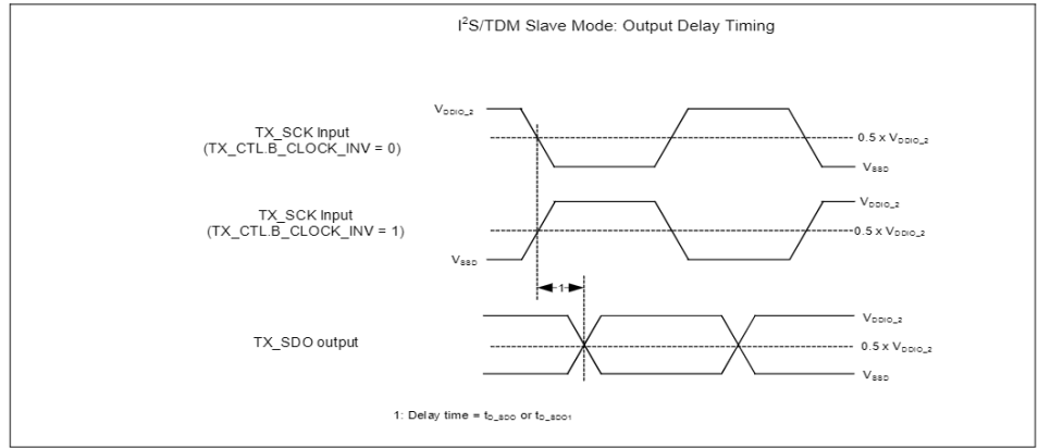
Figure 26-41 Slave output delay
