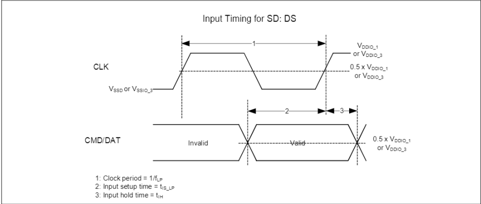
Figure 26-32 SD default speed input timing
