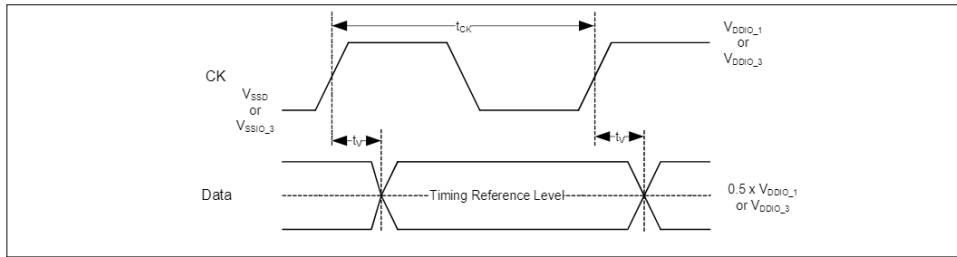
Figure 26-44 SDR read timing reference level
