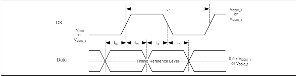
Figure 26-49 HYPERBUS™ timing reference level
