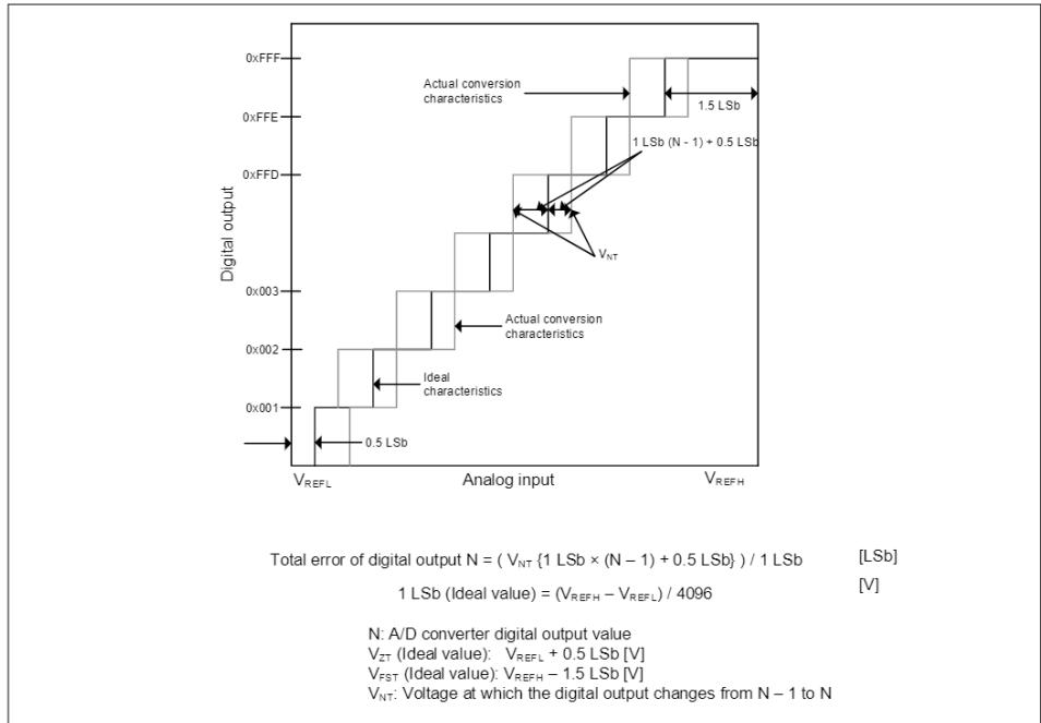
Figure 26-4 ADC characteristics and error descriptions
