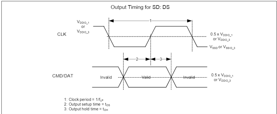
Figure 26-33 SD default speed output timing
