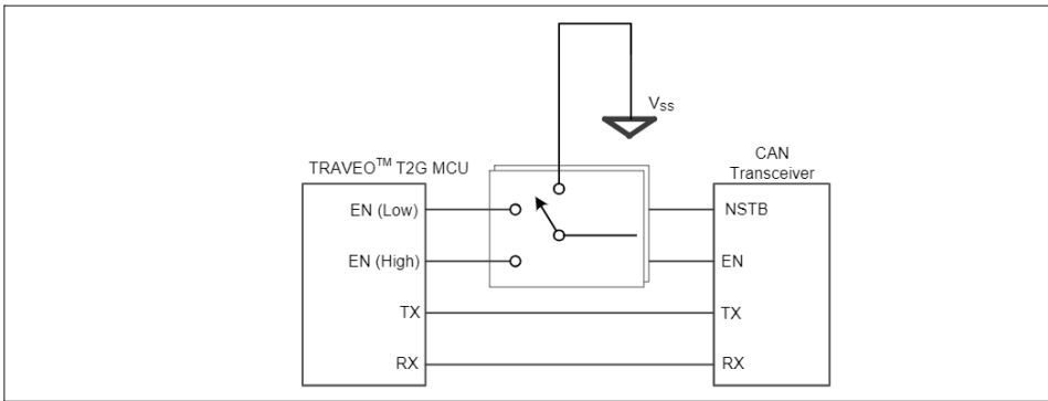
Figure 29-2 MCU to CAN transceiver connections
