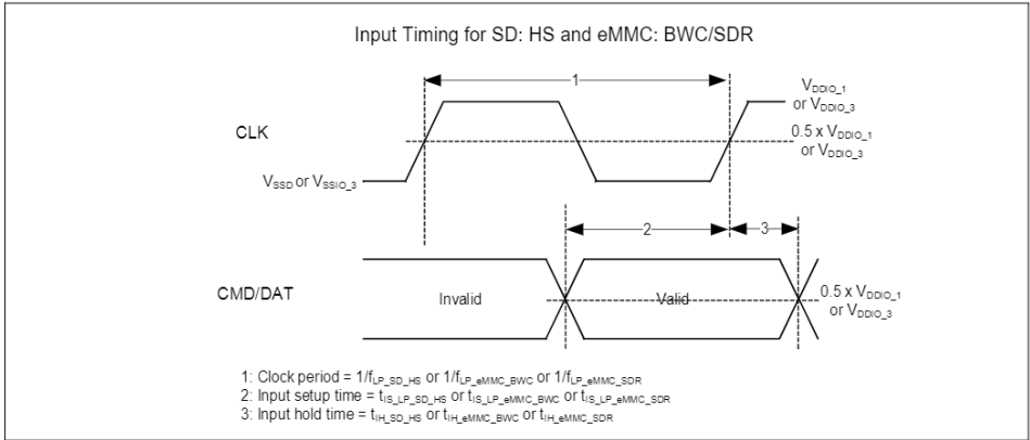
Figure 26-34 SD high-speed and eMMC BWC/SDR input timing
