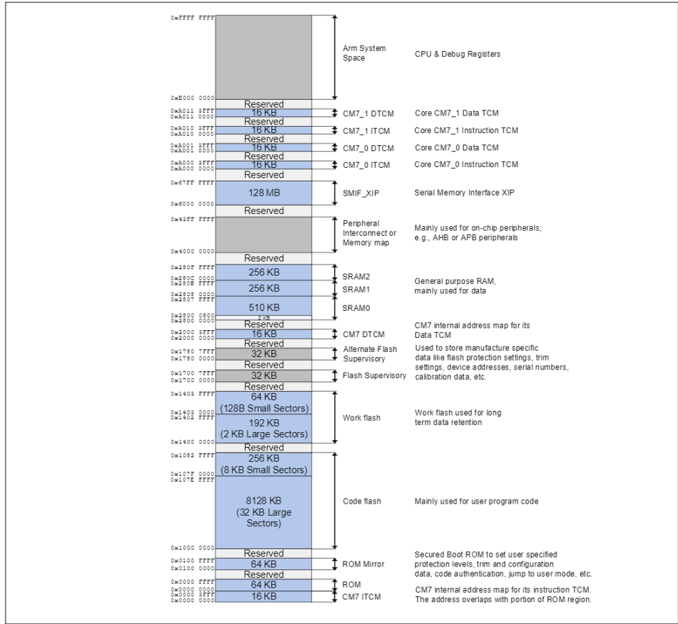
Figure 4-1 CYT4BF address map [13, 14]
