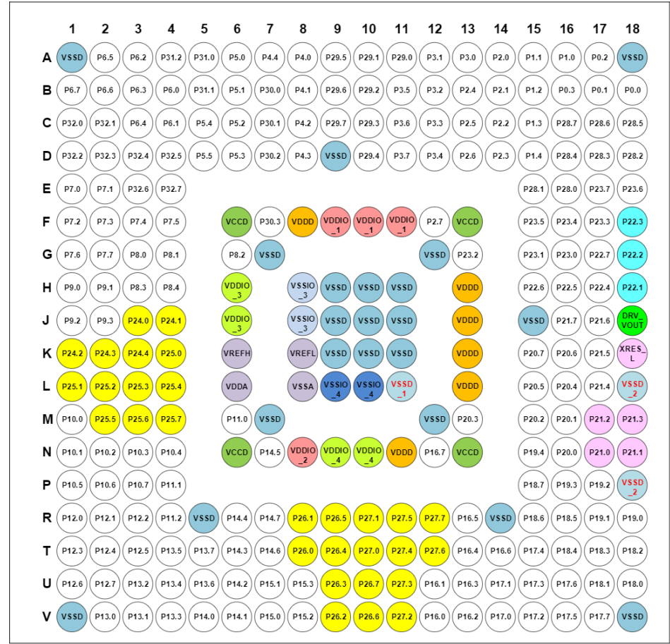
Figure 9-3 272-BGA ball map
