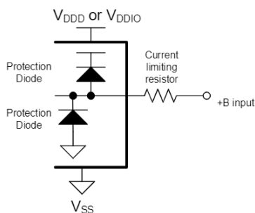
Figure 26-1 Example of a recommended circuit [45]
