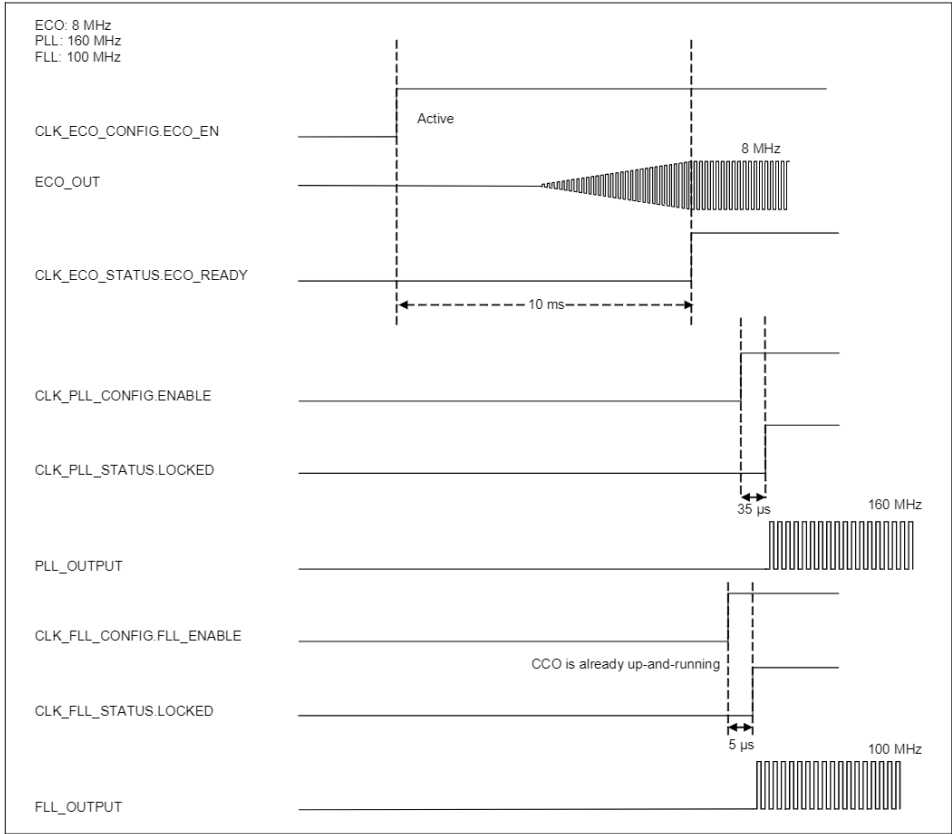
Figure 26-24 ECO to PLL or FLL diagram
