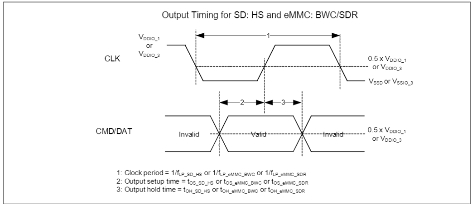
Figure 26-35 SD high-speed and eMMC BWC/SDR output timing
