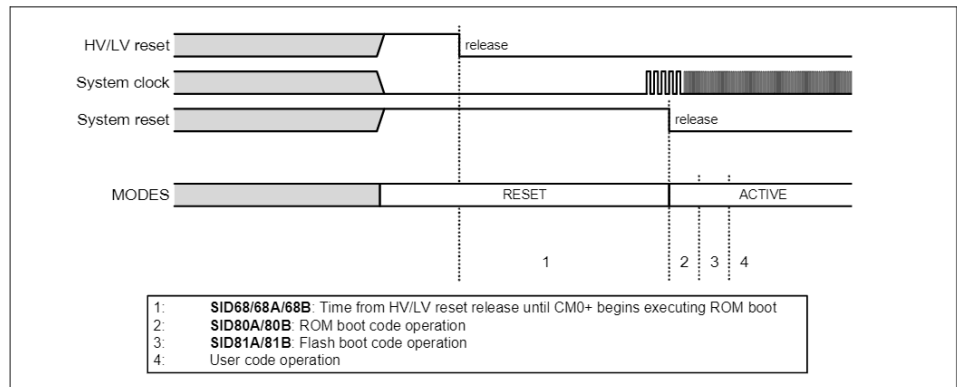
Figure 26-3 Reset sequence
