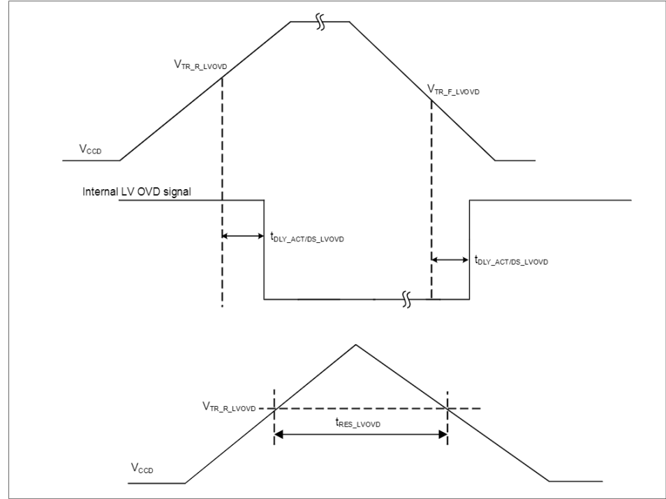
Figure 26-19 Low-voltage OVD specifications
