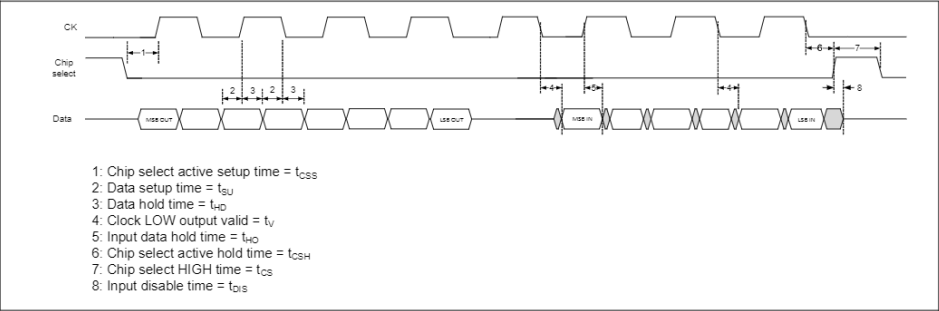
Figure 26-48 DDR write and read timing diagram
