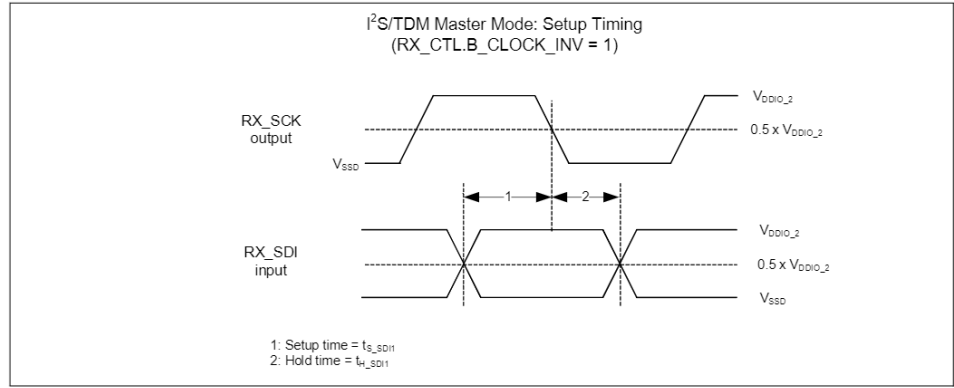
Figure 26-40 Master setup with clock inversion
