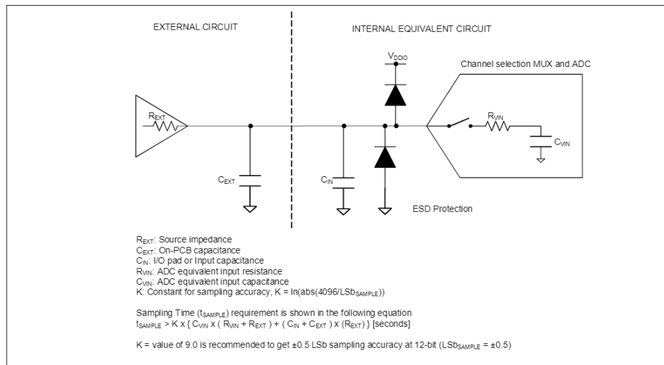
Figure 26-6 ADC equivalent circuit for analog input
