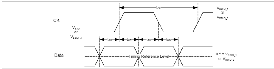
Figure 26-45 DDR write timing reference level
