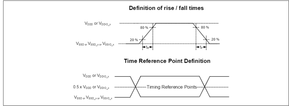
Figure 26-7 AC timings specifications
