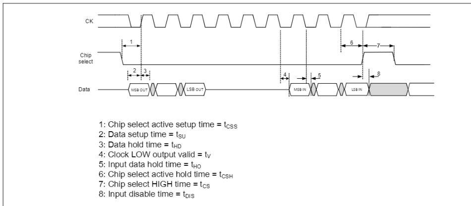
Figure 26-47 SDR write and read timing diagram
