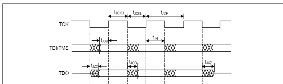
Figure 26-21 JTAG specifications
