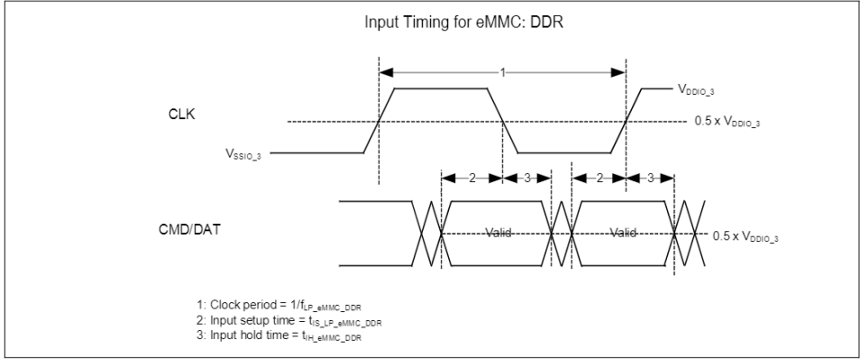
Figure 26-36 eMMC DDR input timing
