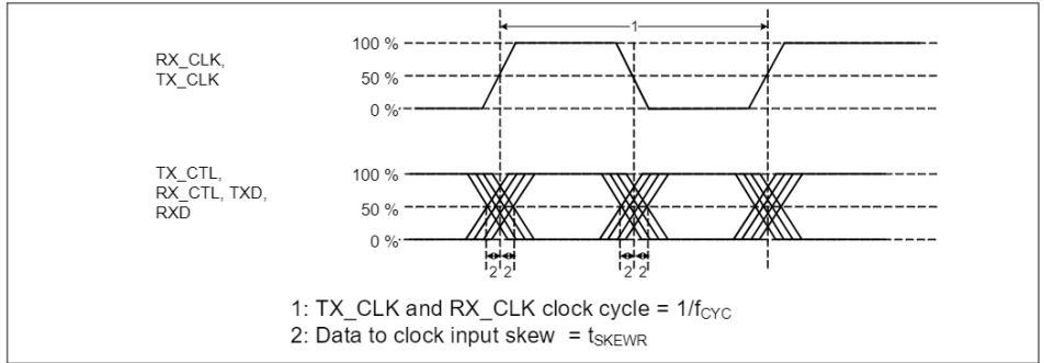
Figure 26-31 RGMII Rx timing diagram
