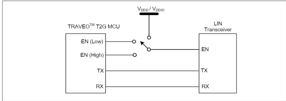
Figure 29-3 MCU to LIN transceiver connections
