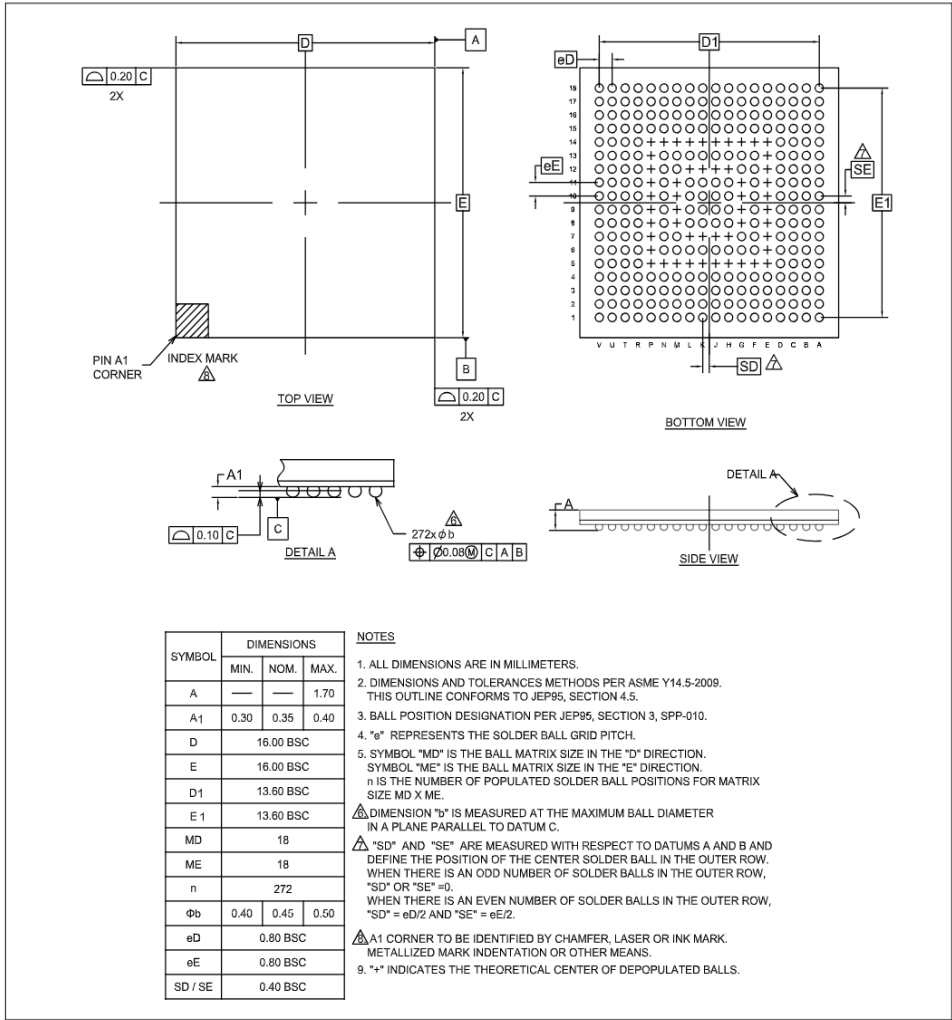
Figure 28-2 Package outline - 272-BGA
