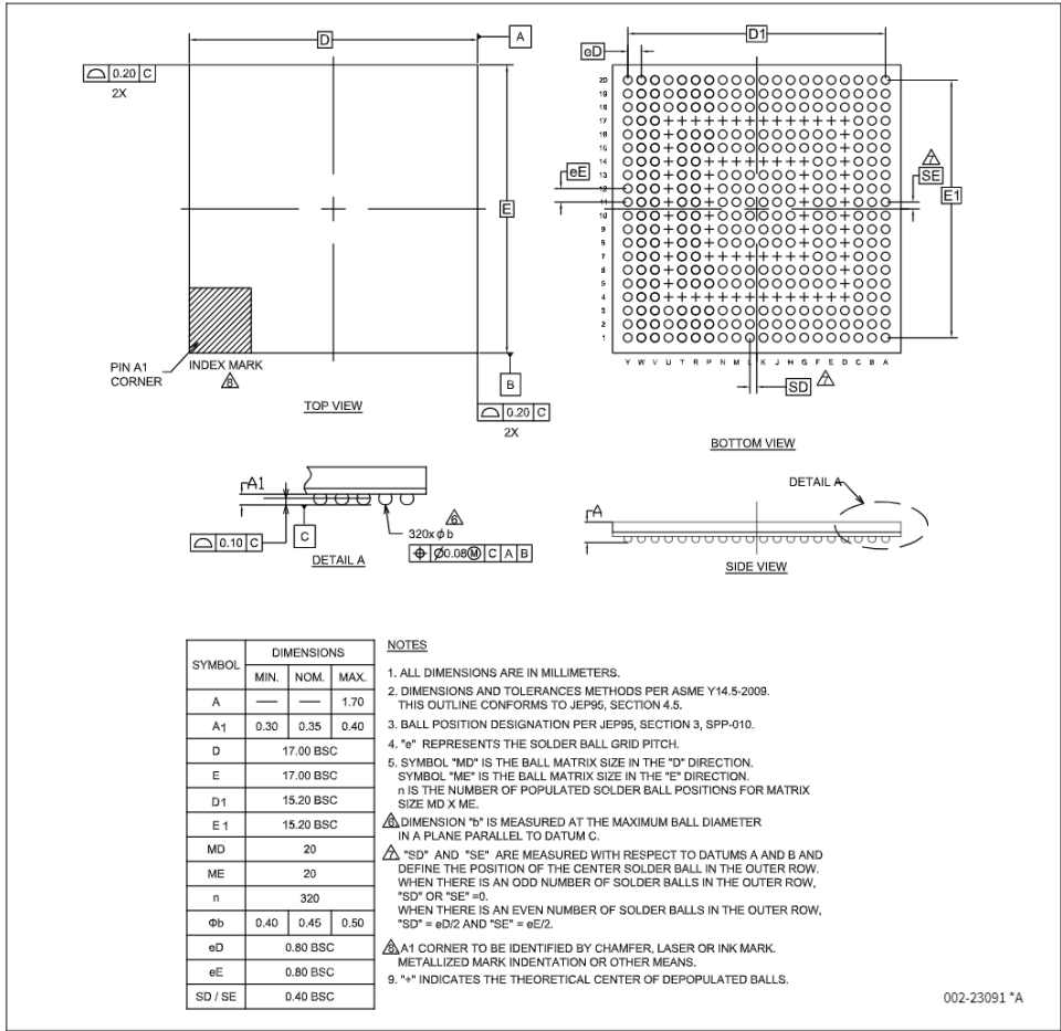
Figure 28-3 Package outline - 320-BGA
