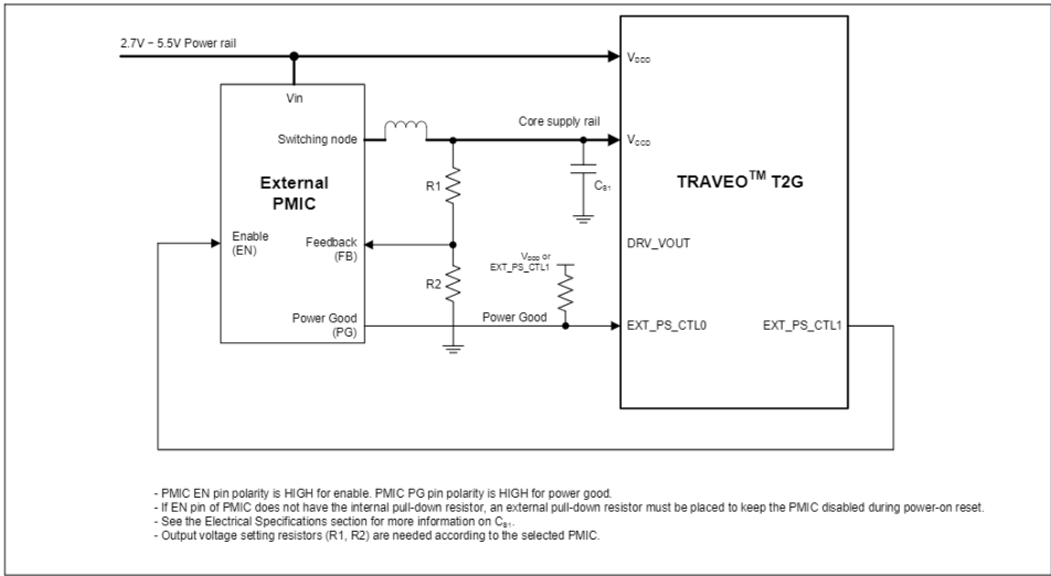
Figure 3-2 Sample core external regulator with PMIC/LDO
