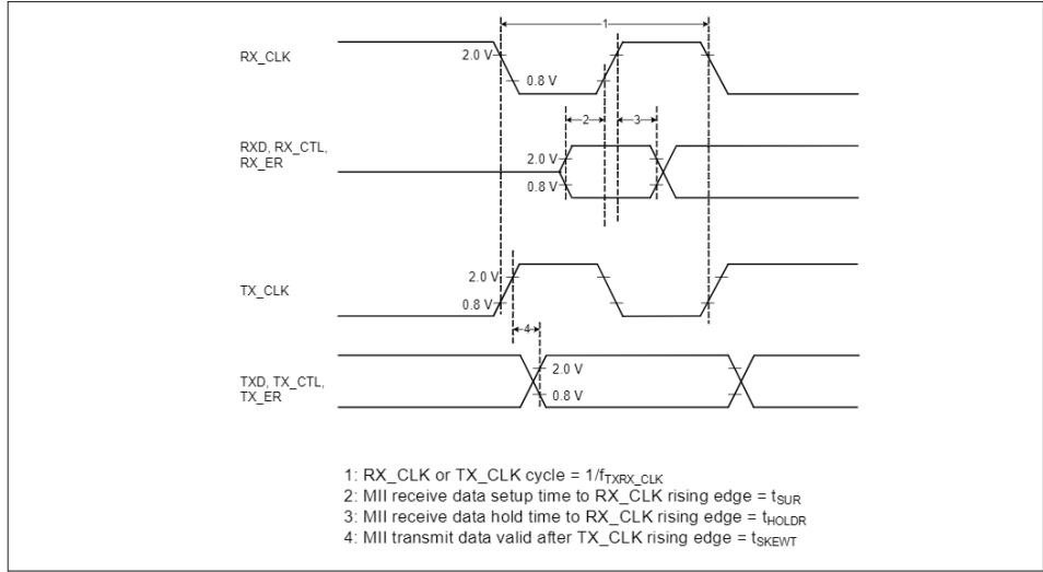
Figure 26-26 MII timing diagram
