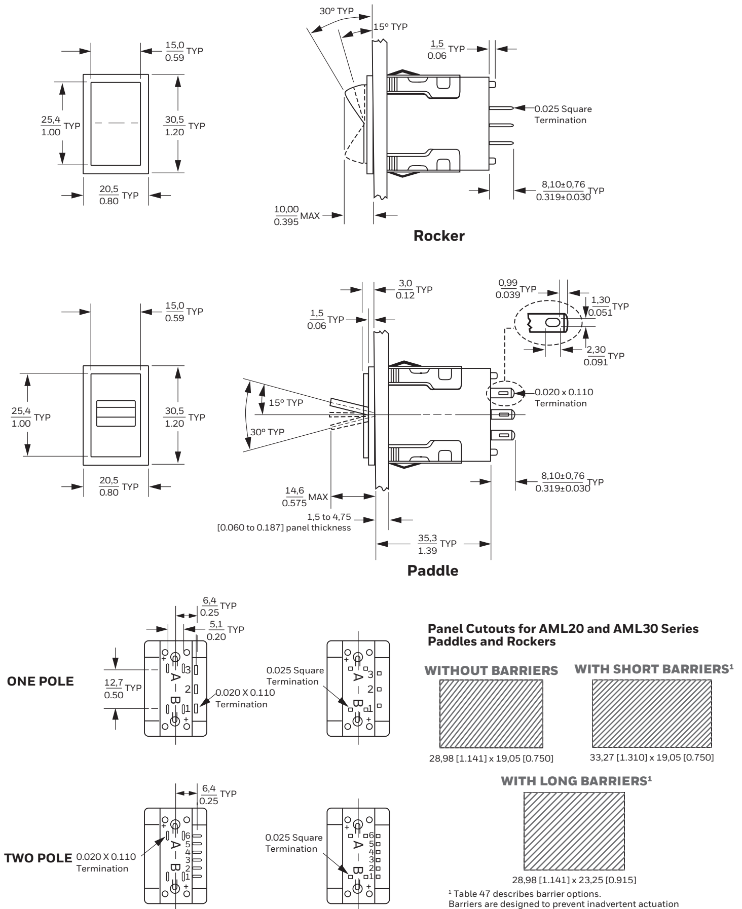
Figure 23. AML23 and AML24 Series Dimensions mm [in] or mm\in
