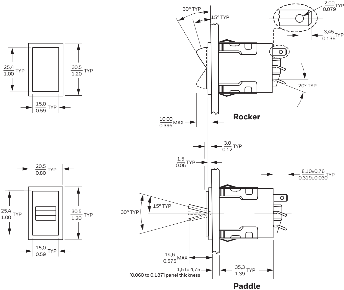
Figure 28. AML33 and AML34 Series Dimensions
