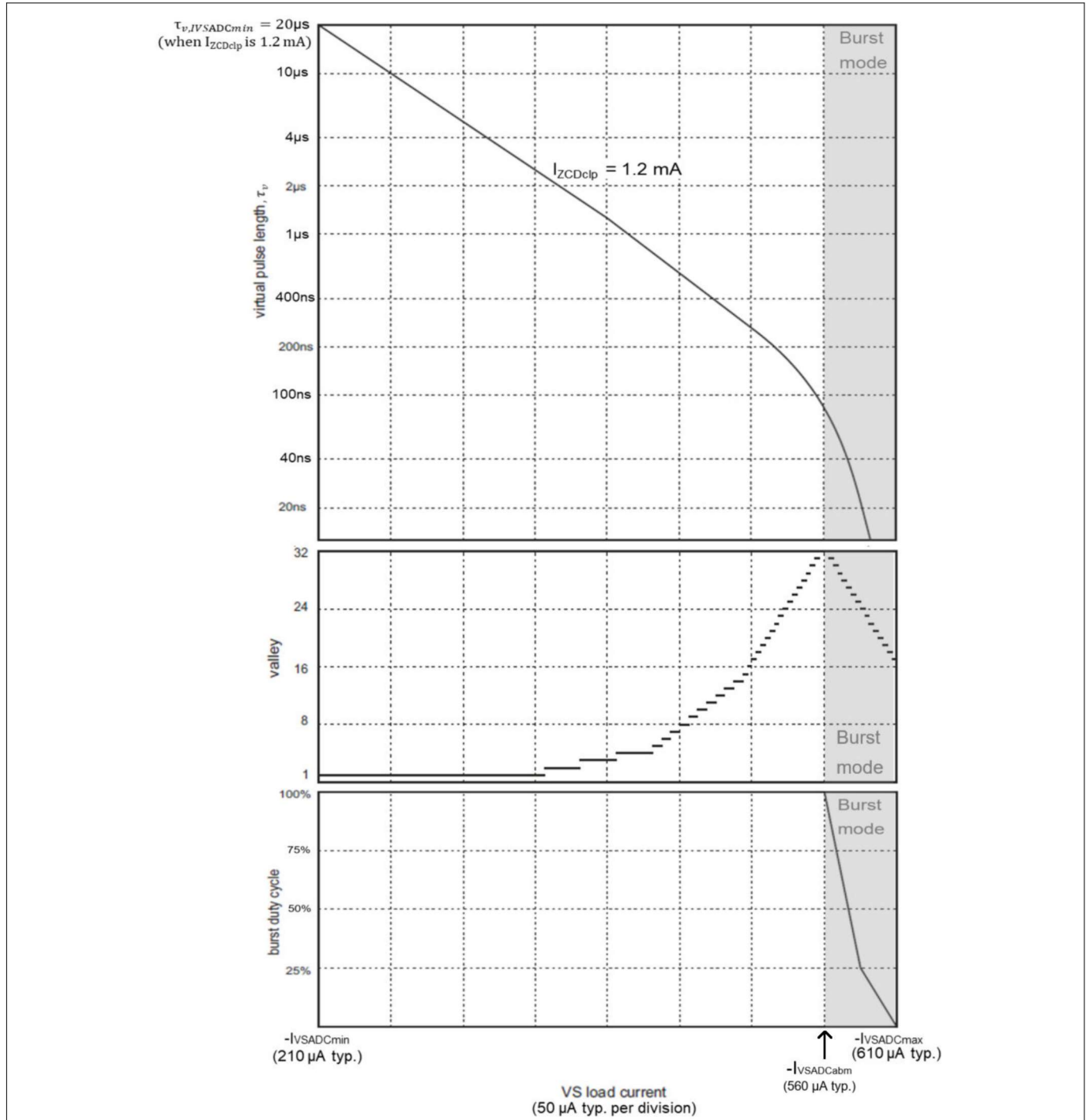
Figure 12 Virtual pulse length mapping (based on I_{ZCDclp} = 1.2 mA as an example), valley number mapping and burst mode mapping
