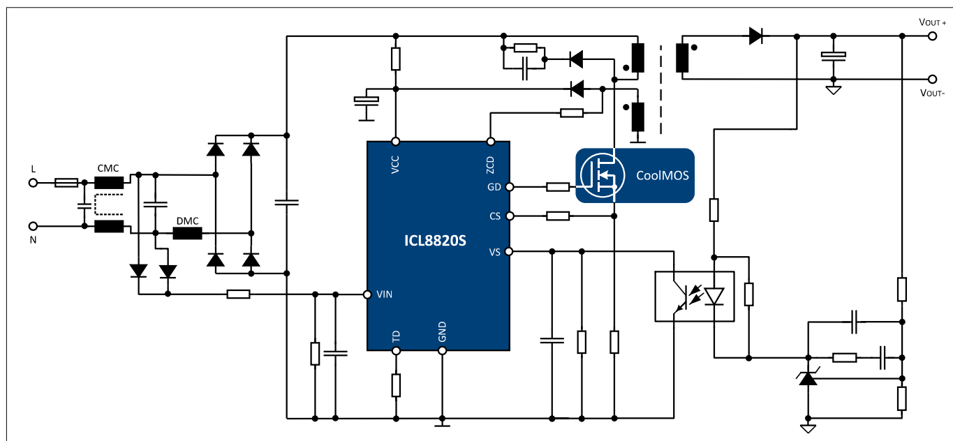
Figure 1 Flyback-SSR-CV
