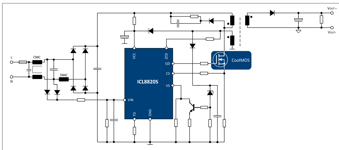
Figure 2 Flyback-PSR-CV
