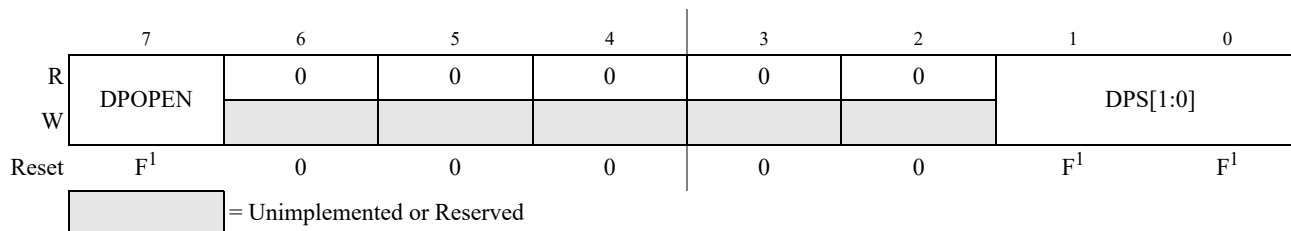
Figure 19-15. EEPROM Protection Register (EPROT)
