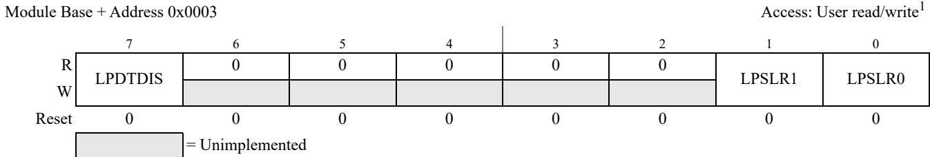
Figure 16-6. LIN Slew Rate Mode Register (LPSLRM)
