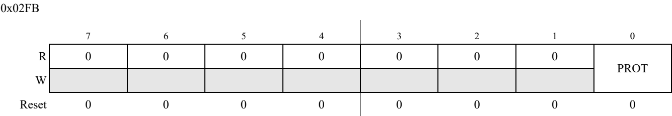
Figure 4-31. S12CPMU_UHV_V8 Protection Register (CPMUPROT)
