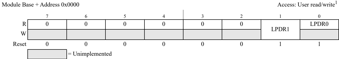
Figure 16-3. Port LP Data Register (LPDR)
