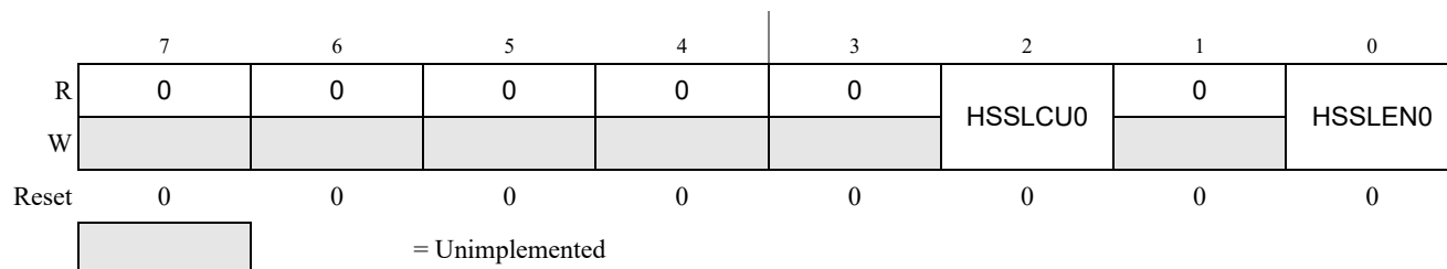
Figure 14-4. HSDRV1C Slew Rate Control Register (HSSLR)
