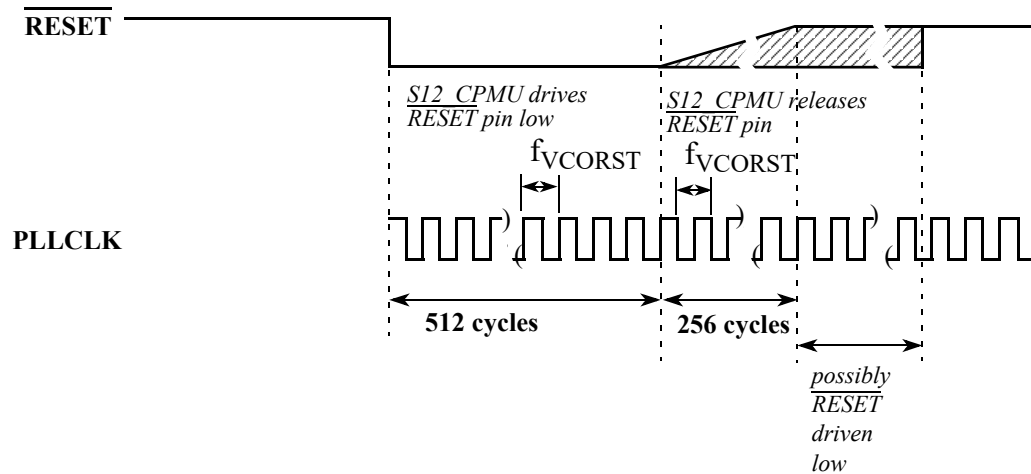
Figure 4-39. RESET Timing
