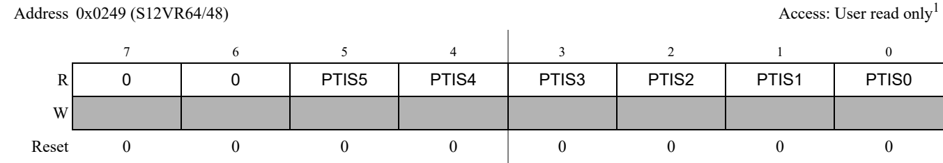
Figure 2-20. Port S Input Register (PTIS - S12VR64/48)
