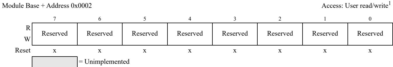
Figure 16-5. LIN Test register
