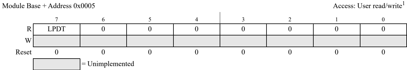
Figure 16-8. LIN Status Register (LPSR)
