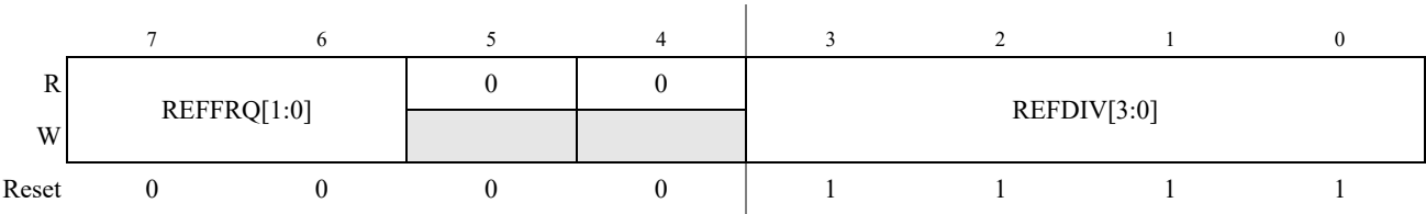
Figure 4-5. S12CPMU_UHV_V8 Reference Divider Register (CPMUREFDIV)
