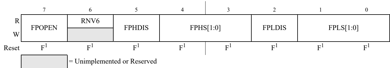
Figure 18-12. Flash Protection Register (FPROT)
