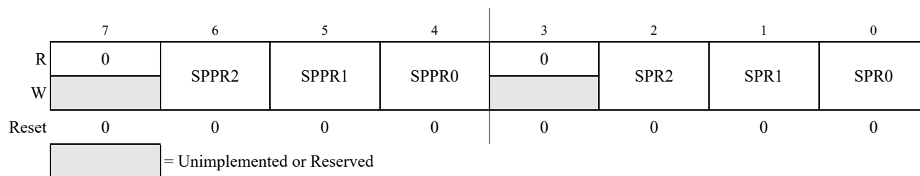
Figure 11-5. SPI Baud Rate Register (SPIBR)
