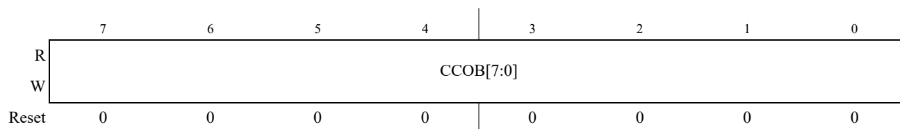
Figure 19-17. Flash Common Command Object Low Register (FCCOBLO)
