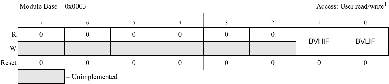
Figure 17-7. BATS Interrupt Flag Register (BATIF)
