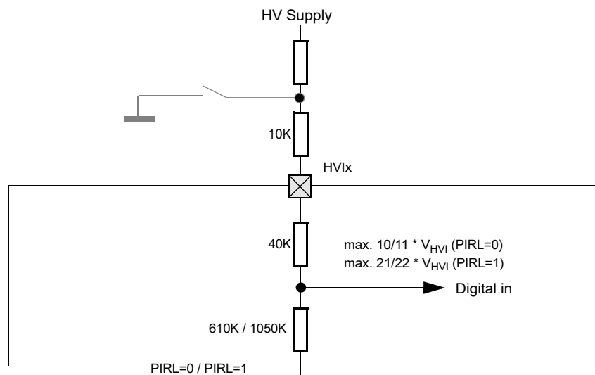
Figure 2-74. Digital Input Read with Pulldown Enabled
