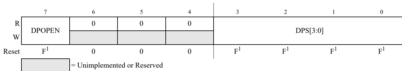
Figure 18-14. EEPROM Protection Register (EPROT)
