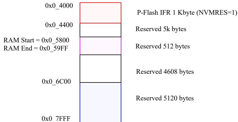
Figure 18-2. Memory Controller Resource Memory Map (NVMRES=1)
