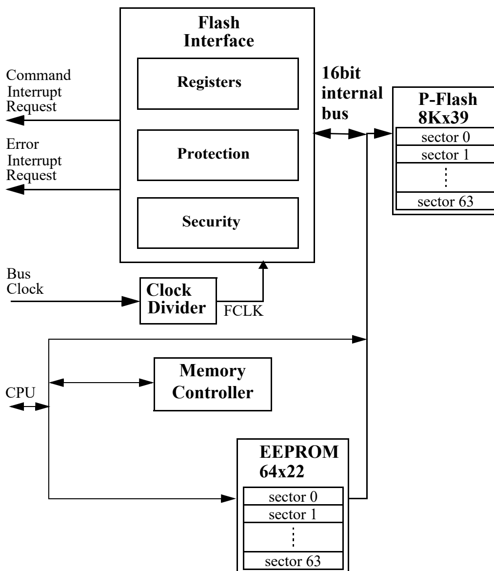
Figure 19-1. FTMRG32K128 Block Diagram
