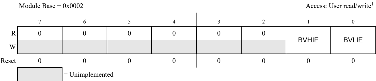
Figure 17-6. BATS Interrupt Enable Register (BATIE)
