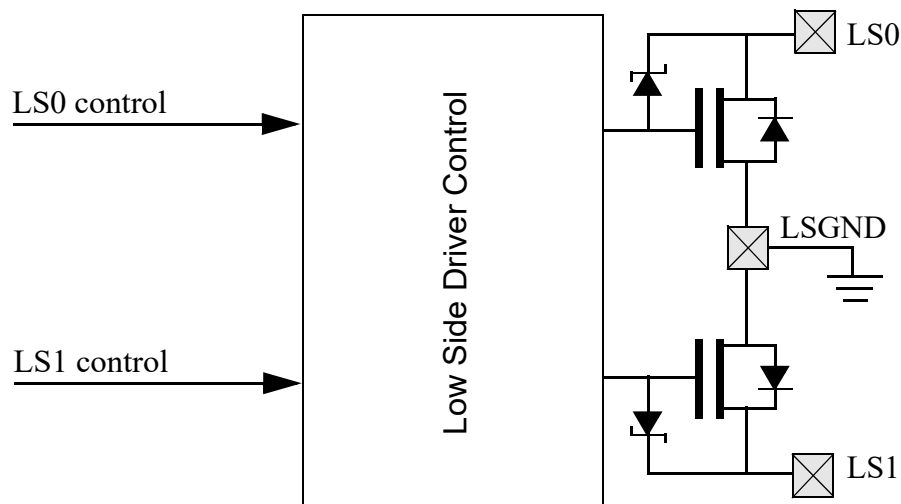
Figure 15-1. LSDRV Block Diagram
