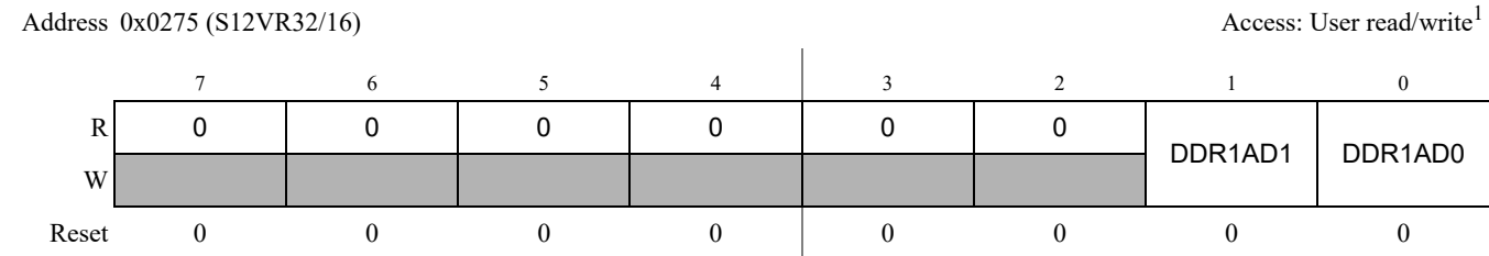
Figure 2-61. Port AD Data Direction Register (DDR1AD - S12VR32/16)
