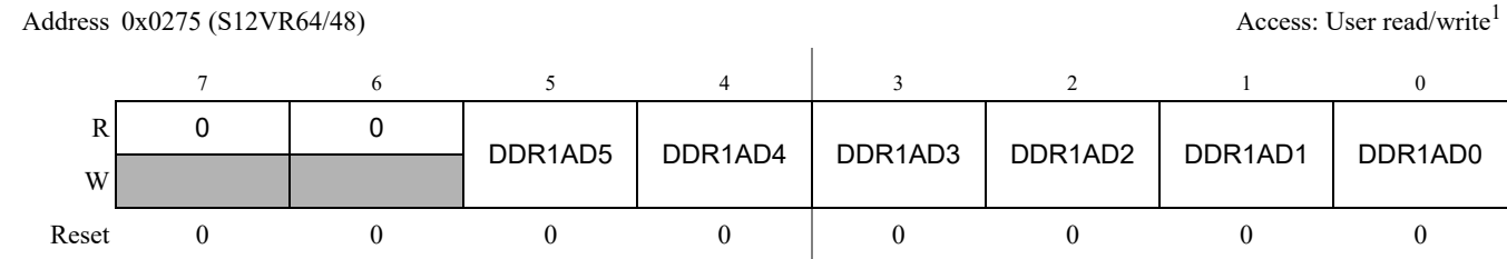
Figure 2-60. Port AD Data Direction Register (DDR1AD - S12VR64/48)
