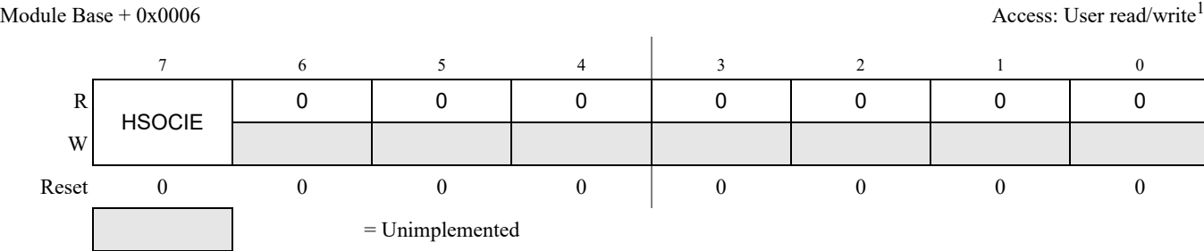
Figure 14-7. HSDRV1C Interrupt Enable Register (HSIE)
