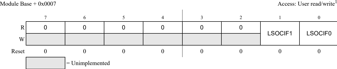
Figure 15-6. LSDRV Interrupt Flag Register (LSIF)
