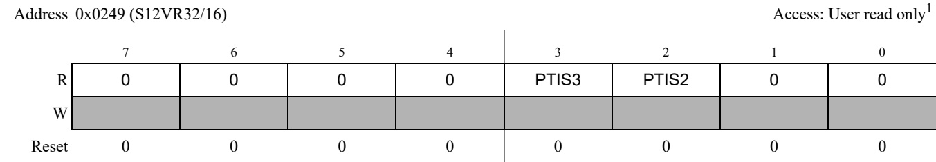
Figure 2-21. Port S Input Register (PTIS - S12VR32/16)
