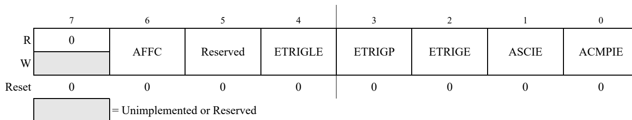
Figure 8-5. ATD Control Register 2 (ATDCTL2)
