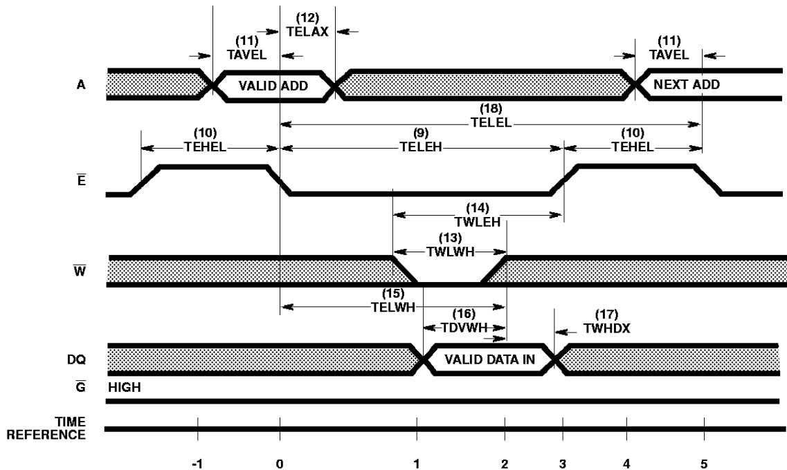
FIGURE 2. WRITE CYCLE
