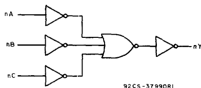
92CS-37990R1 LOGIC DIAGRAM
