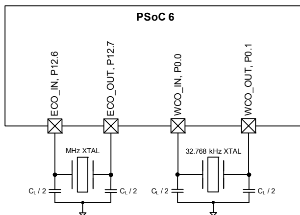
Figure 4. Oscillator Circuits
