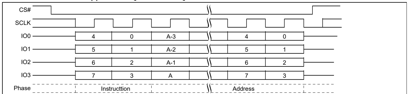
Figure 94 EES QPI mode command sequence [57]
