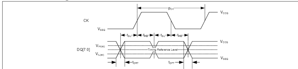
Figure 56 Input timing reference levels
