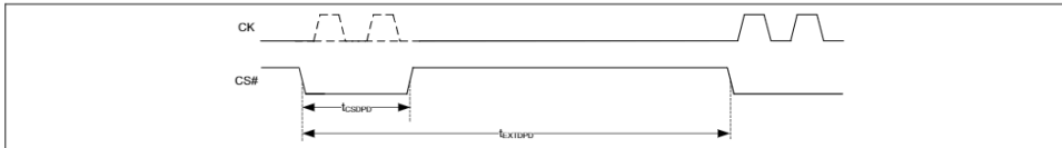
Figure 46 Exit DPD mode
