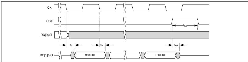
Figure 61 SPI output timing
