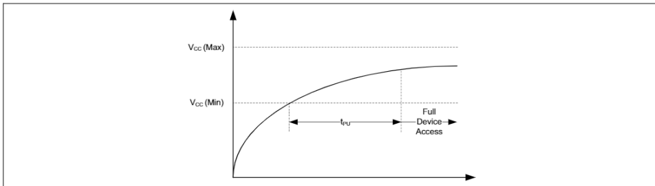
Figure 47 Power up
