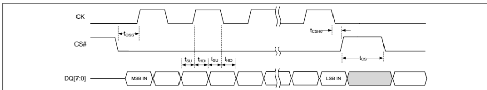
Figure 62 HYPERBUS™ DDR input timing
