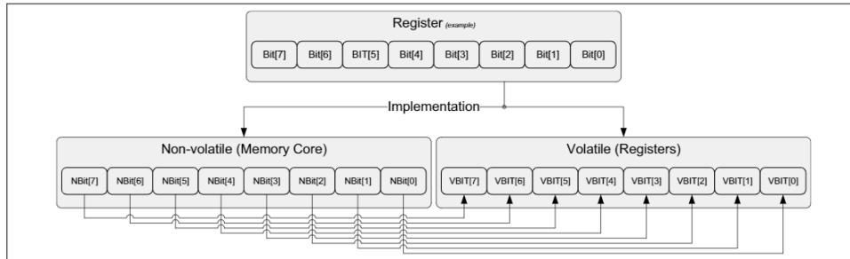
Figure 50 Register structure
