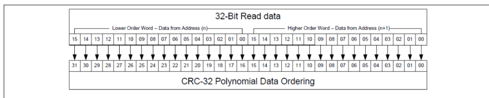
Figure 25 CrC-32 data ordering
