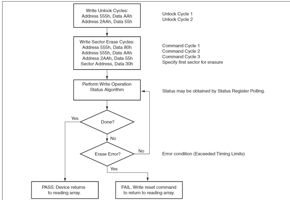
Figure 37 Sector erase operation
