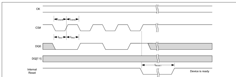
Figure 44 CS# signaling reset protocol
