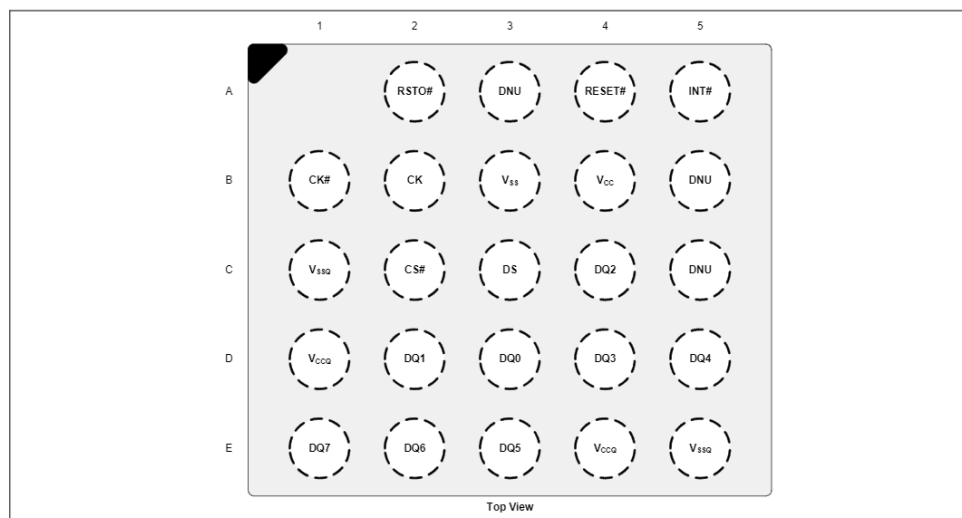
Figure 1 24-ball BGA pinout configuration [1]
