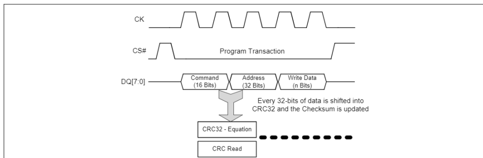
Figure 24 Program CRC protection
