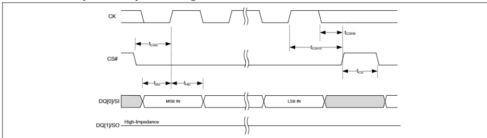
Figure 60 SPI input timing
