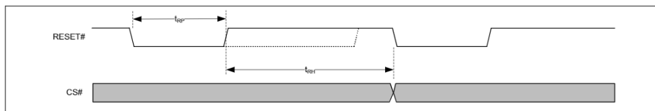
Figure 41 Hardware reset using RESET# input (Back to back hardware reset)
