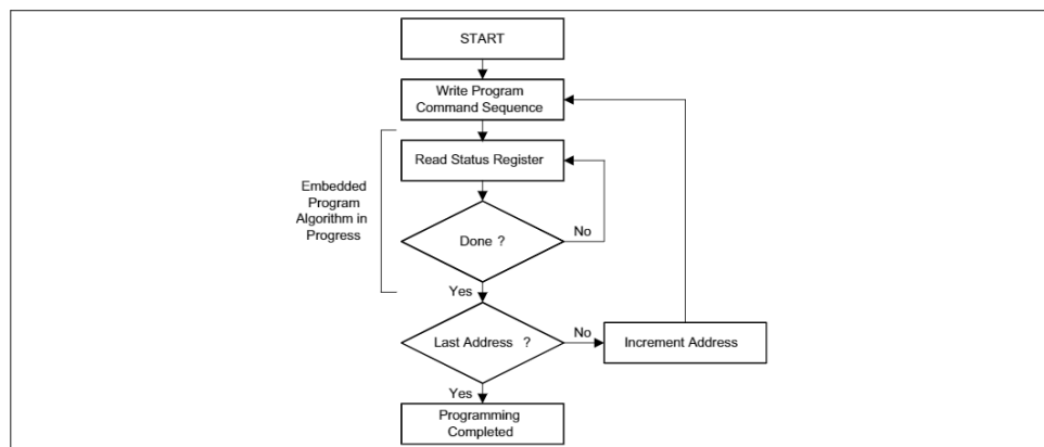
Figure 35 Word program operation
