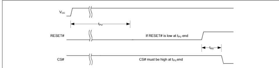
Figure 42 Reset LOW at the end of POR
