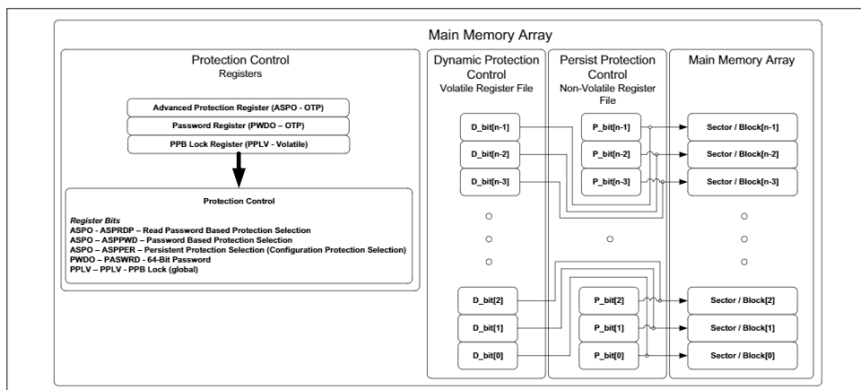
Figure 27 Advanced sector protection (Nonvolatile)
