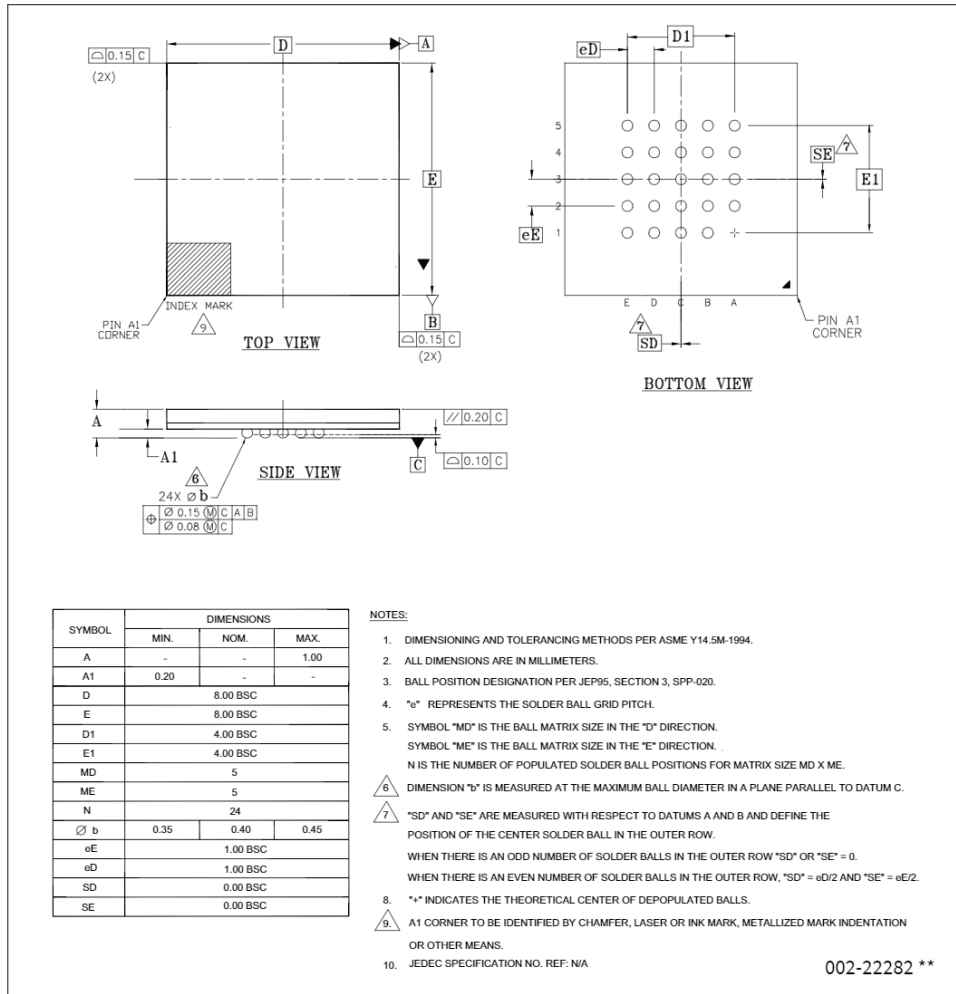
Figure 65 Ball grid array 24-ball 8 x 8 mm (VAC024)
