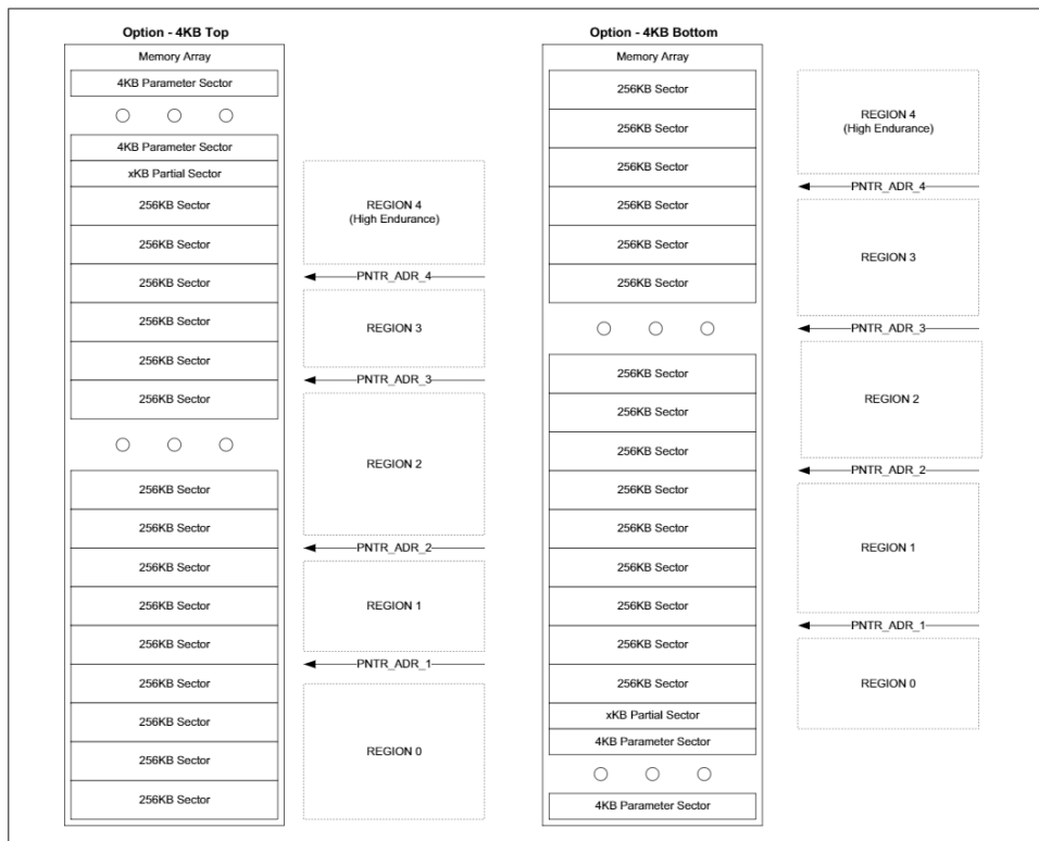
Figure 20 Infineon® Endurance Flex architecture overview
