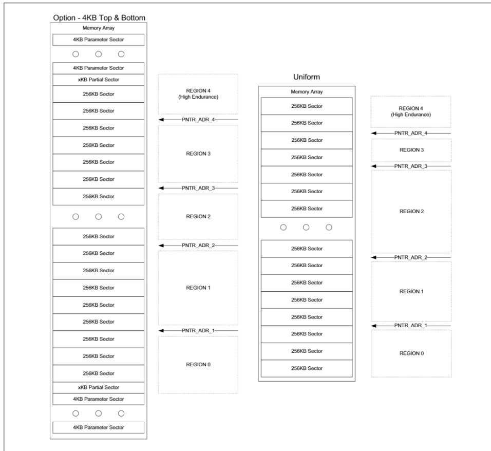
Figure 21 Infineon® Endurance Flex architecture overview (Continued)
