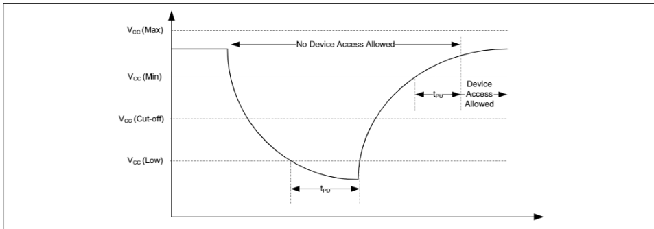
Figure 48 Power down and voltage drop
