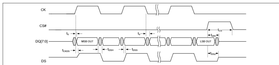
Figure 63 HYPERBUS™ DDR output timing
