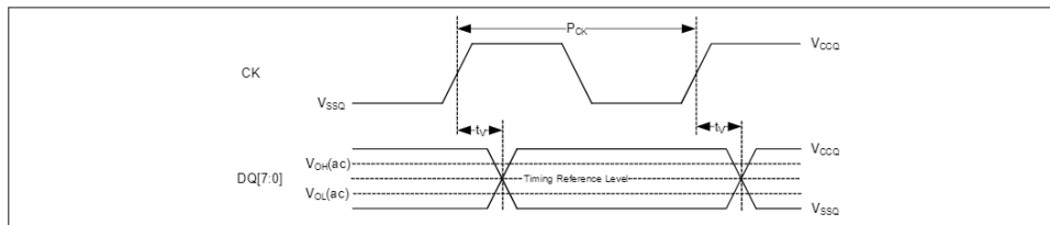
Figure 57 SDR output timing reference level
