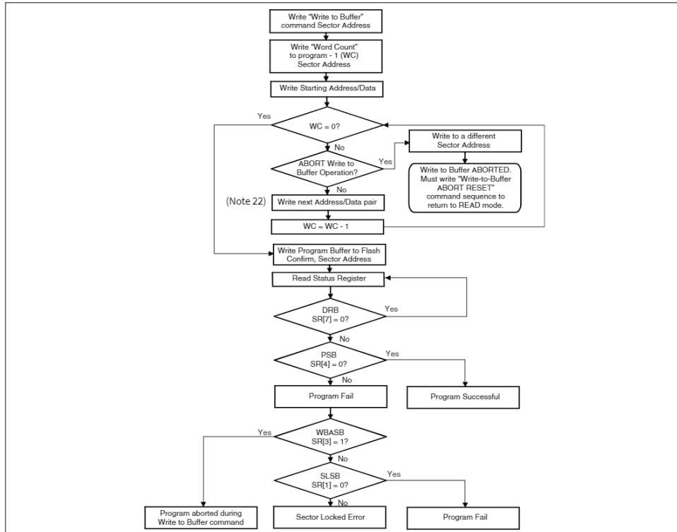
Figure 36 Write buffer programming operation with status register
