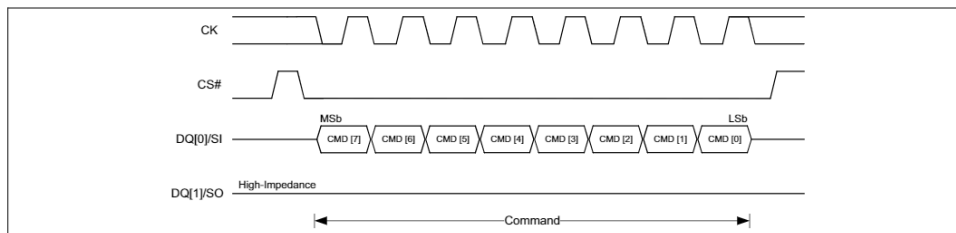
Figure 5 SPI transaction with command input
