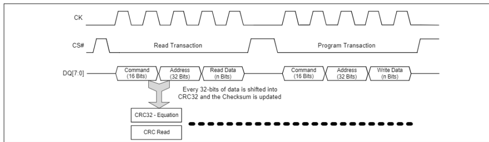
Figure 22 CRC calculation overview
