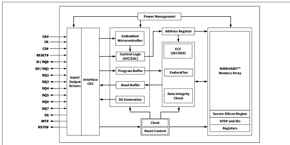
Figure 2 Logic block diagram
