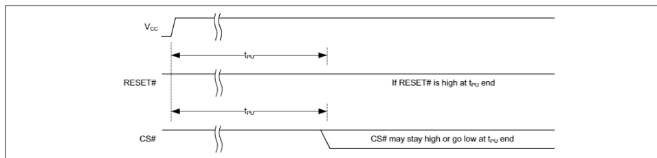
Figure 43 Reset HIGH at the end of POR
