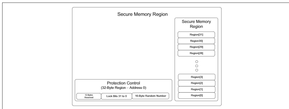
Figure 31 OTP protection (Nonvolatile)
