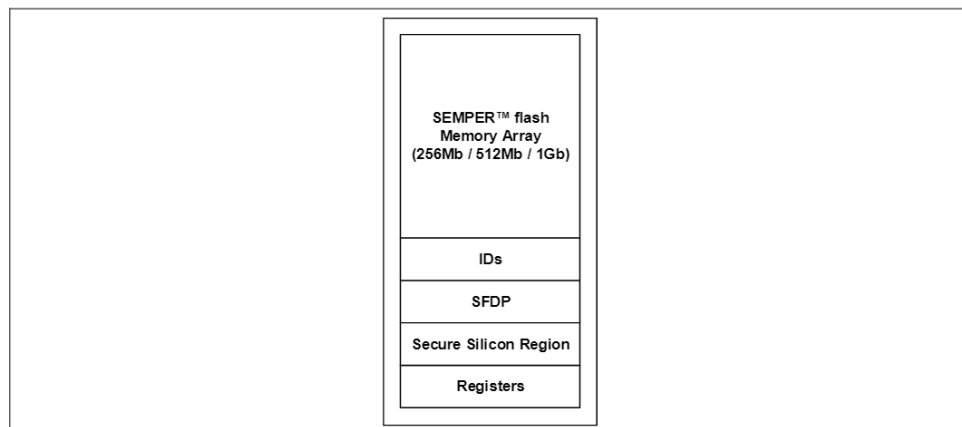
Figure 18 SEMPER™ Flash address space map overview
