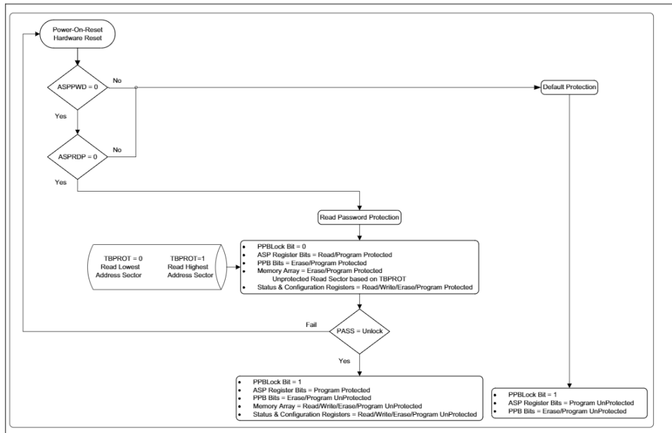
Figure 30 Read password protection scheme flowchart
