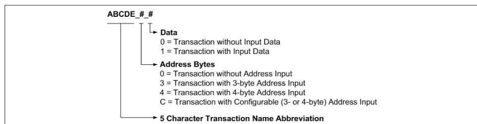
Figure 17 Legacy (x1) SPI transaction naming convention
