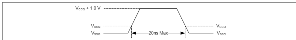
Figure 53 Maximum positive overshoot waveform
