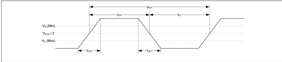
Figure 59 Clock timing
