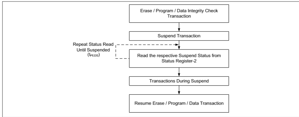
Figure 38 Suspend and resume sequence
