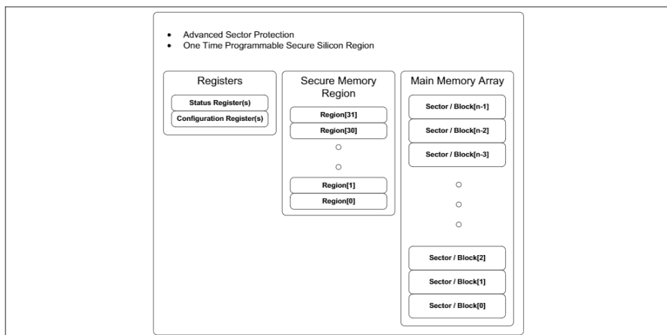
Figure 26 Data protection and security (Write/Program/Erase) schemes
