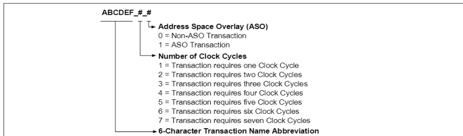
Figure 16 HYPERBUS™ transaction naming convention
