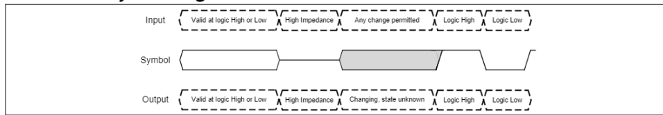
Figure 55 Waveform element meanings
