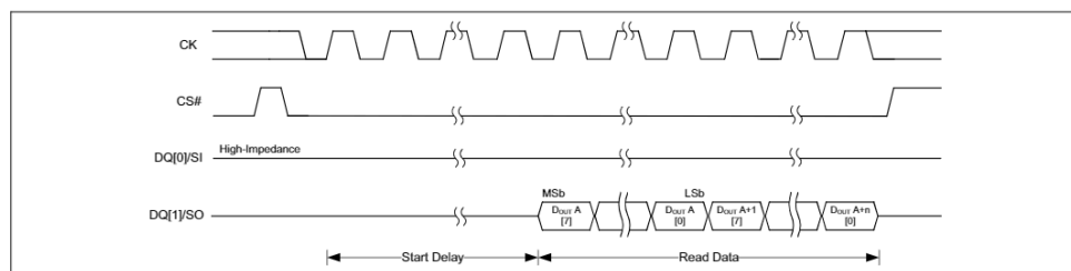
Figure 13 SPI transaction with output data sequence (AutoBoot)
