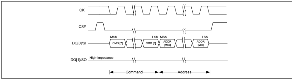
Figure 6 SPI transaction with command and address input
