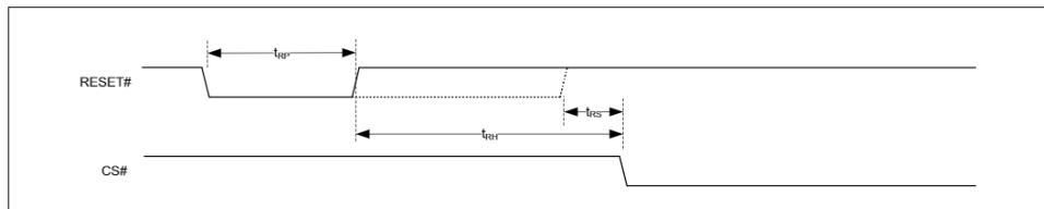
Figure 39 Hardware reset using RESET# input (Reset pulse = t_{RP} (Min))
