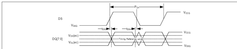
Figure 58 DDR output timing reference level
