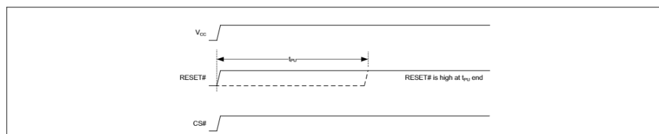
Figure 45 Enter DPD mode upon power-up or reset
