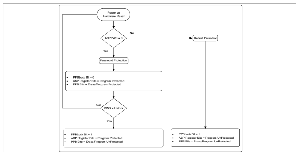
Figure 29 Password protection scheme flowchart
