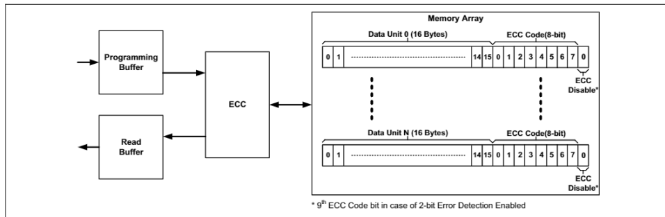
Figure 19 16-Byte ECC data unit example
