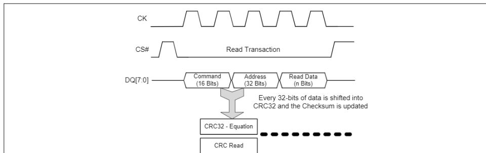
Figure 23 Read CRC protection
