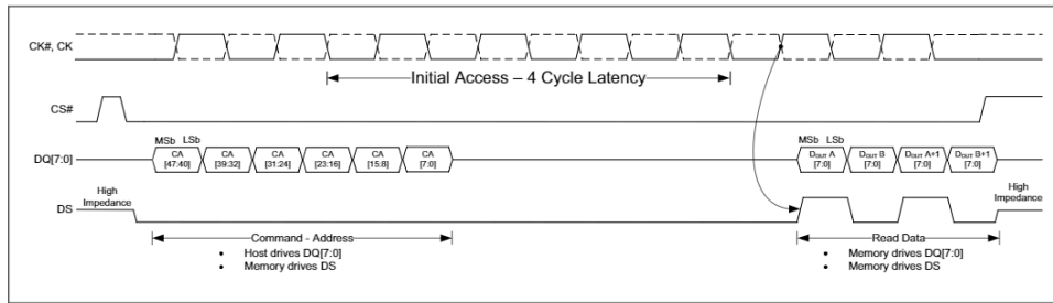
Figure 3 Read operation (Single initial latency) [4, 5, 6, 7, 8]
