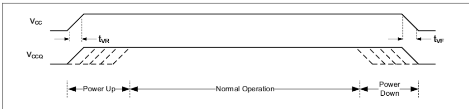
Figure 49 Power up and power down sequence
