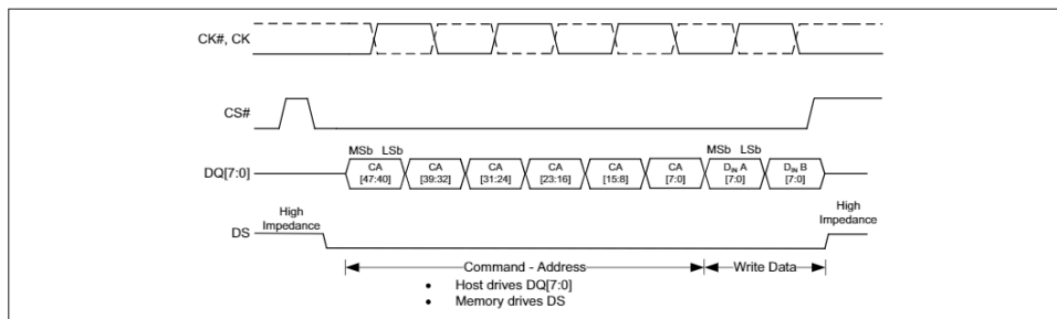
Figure 4 Write operation [4, 9, 10]
