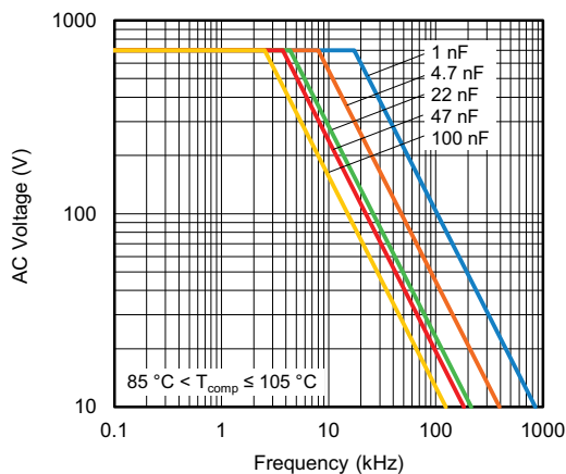
Maximum RMS voltage as a function of frequency (2000 V DC )
