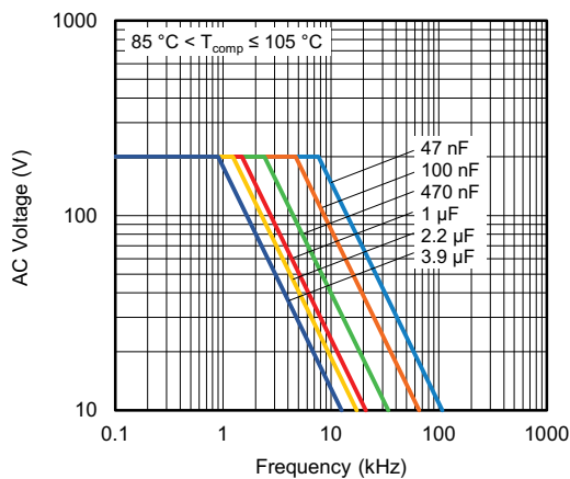
Maximum RMS voltage as a function of frequency (400 V DC )
