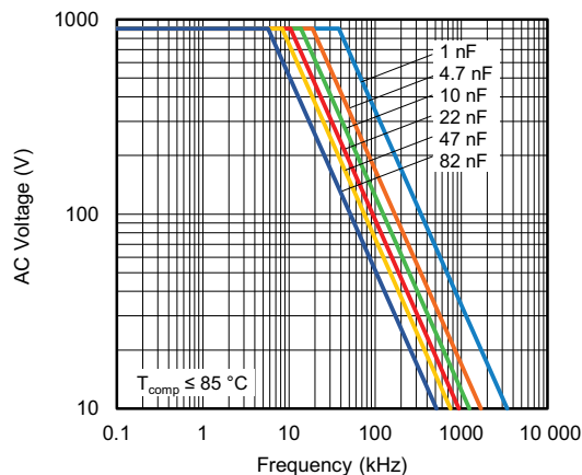
Maximum RMS voltage as a function of frequency (2500 V_{DC} )
