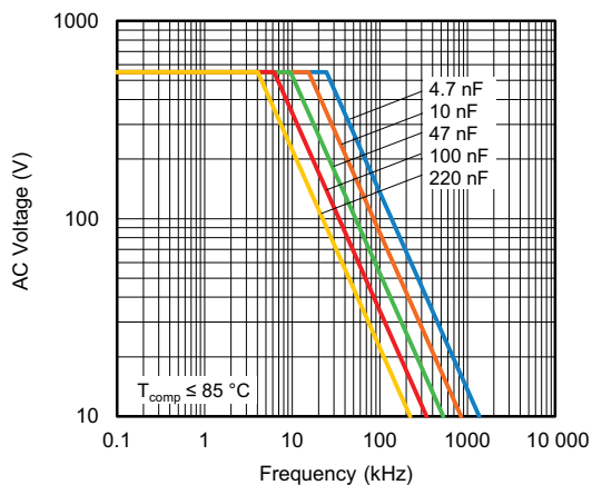
Maximum RMS voltage as a function of frequency (1600 V_{DC} )
