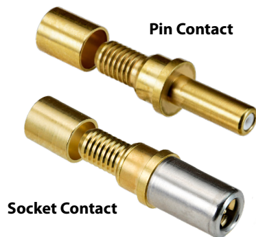
Pin Contact 852-103-01, -02
