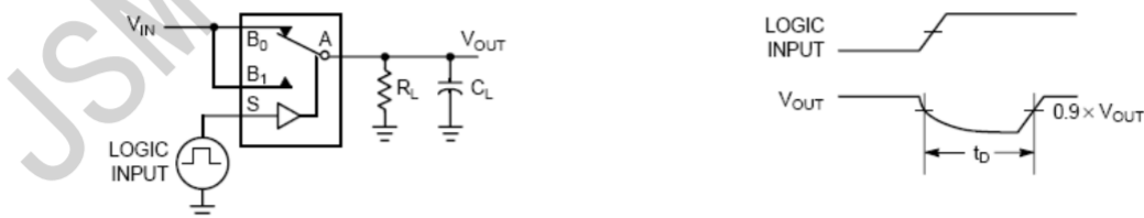
Figure 2. Break Before Make Interval Timing
