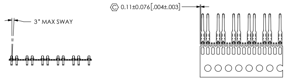
IN PROCESS 3 CUT C-266-XX.X-X CONTACT COMBS (FOR QRF8-018-05.0-X-D-DP-A-GP)
