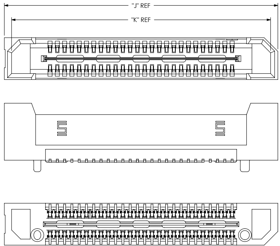
FIG 3 -GP OPTION (QRF8-026-05.0-X-D-A-GP SHOWN) (SAME AS FIG 2 DIFFERENT AS SHOWN)
