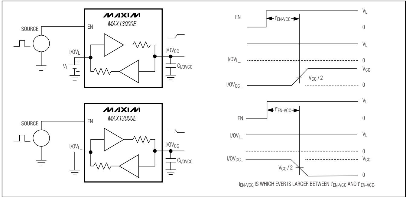
Figure 3. Propagation Delay from I/OV_L to I/OV_{VCC} After EN
