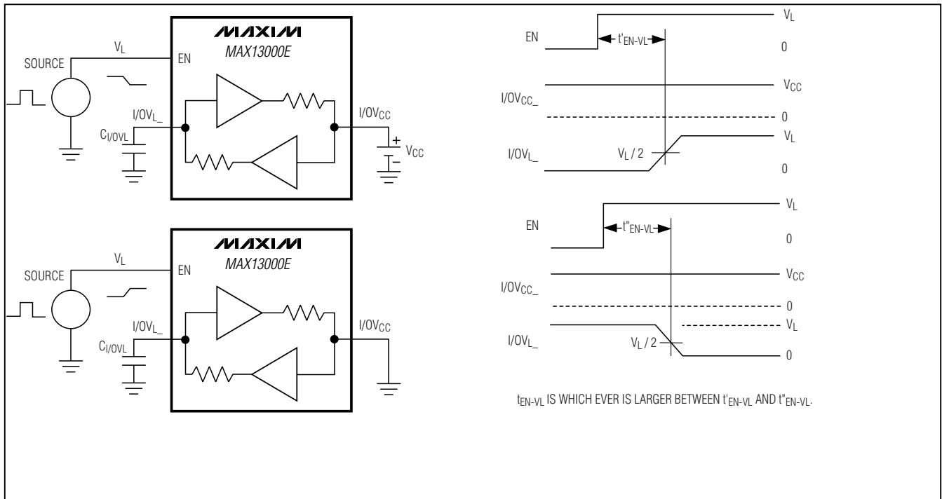
Figure 4. Propagation Delay from I/OV_{VCC} to I/OV_L After EN
