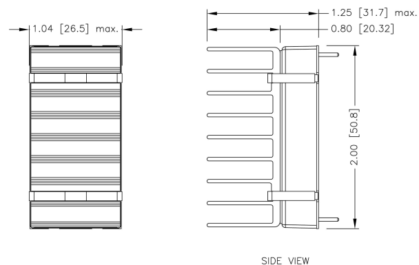
RED60-□□□□□W- HC3 7GA0122P01-F
