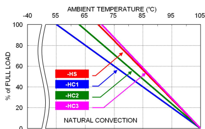
RED60-24S05W Derating Curve With Heat-sink
