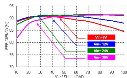
RED60-24S05W Efficiency vs. Output Load
