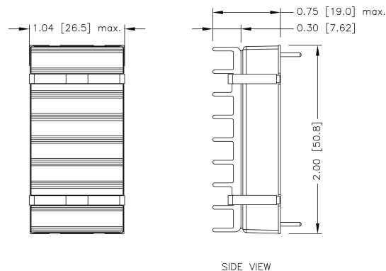
RED60-□□□□□W- HC3 7GA0122P01-F
