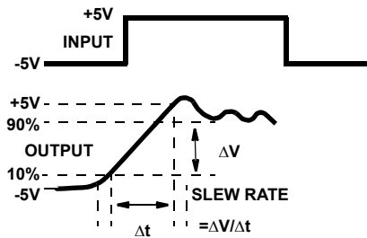
FIGURE 2. SLEW RATE
