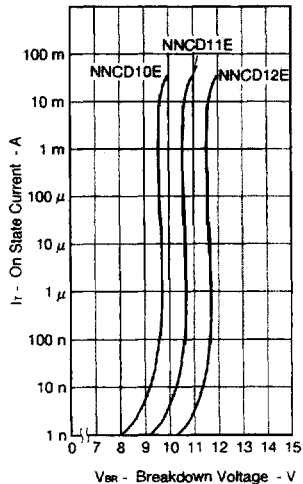
Fig. 3 I_T - V_{BR} CHARACTERISTICS
