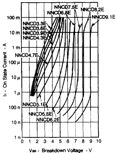
Fig. 2 I_T - V_{BR} CHARACTERISTICS
