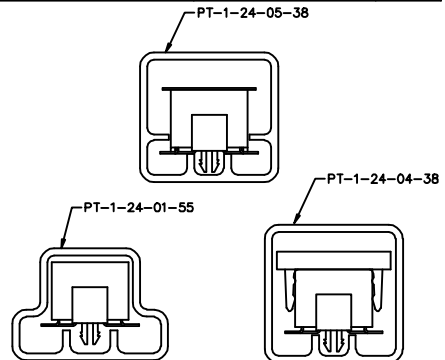
PACKAGING VIEW SCALE .75
