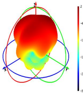
1880 MHz
