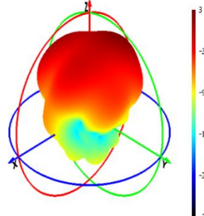
1950 MHz
