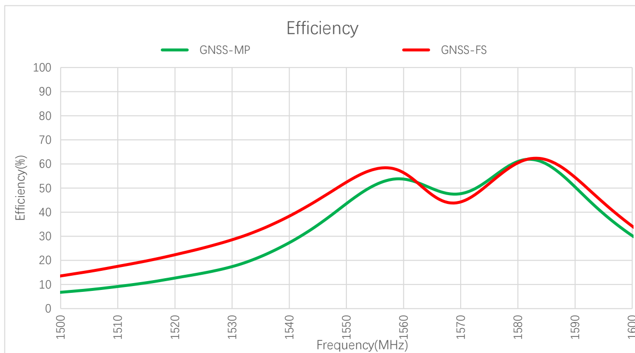
Efficiency (%) - GNSS
