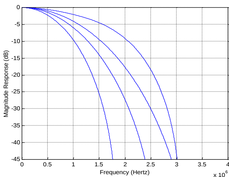
Fig. 6 The Characteristics of Chrominance Low Pass Filter
