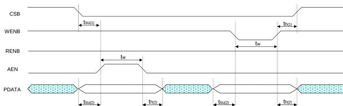
Fig 23. Write Timing Diagram in Parallel Interface
