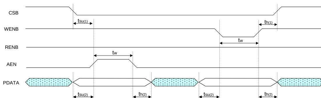
Fig 18 Write mode in Parallel interface
