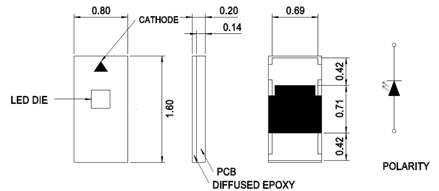
Figure 1: Package Dimensions
