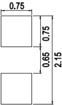
Figure 7: Recommended Soldering Land Pattern
