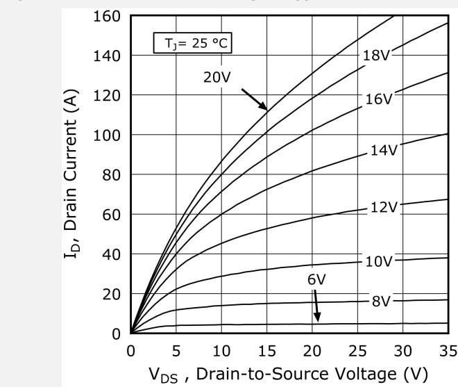
Figure 1-4. Drain Current vs. V_{DS} at V_{GS}
